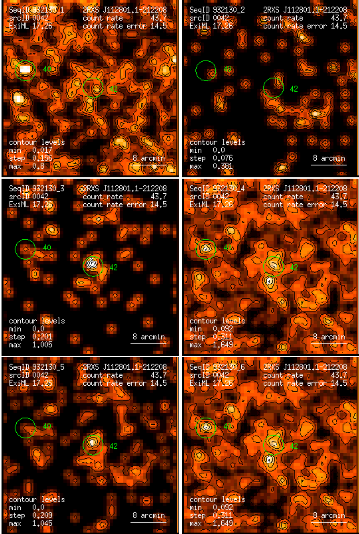
Figure 42: RASS 932130: detection 0042: band rate images, Gaussian filter: (1) PSPC channels 11 – 41, (2) 52 – 90, (3) 91 – 201, (4) 11 – 235, (5) 52 – 201, (6) 11 – 201. Broad band rates in counts/ks. Band rate contour levels in counts/ks/arcmin 2 .
