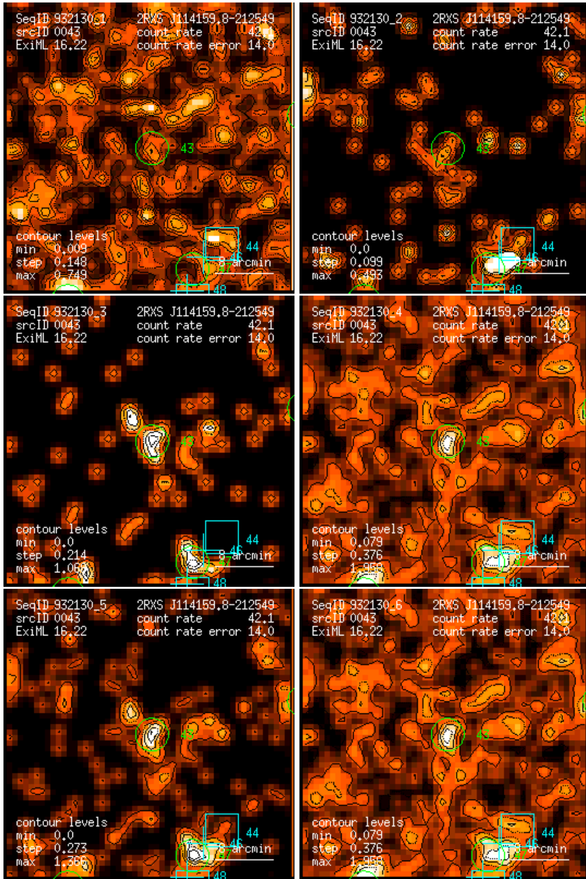
Figure 43: RASS 932130: detection 0043: band rate images, Gaussian filter: (1) PSPC channels 11 – 41, (2) 52 – 90, (3) 91 – 201, (4) 11 – 235, (5) 52 – 201, (6) 11 – 201. Broad band rates in counts/ks. Band rate contour levels in counts/ks/arcmin 2 .
