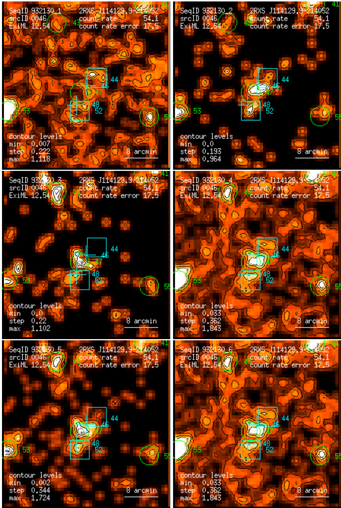
Figure 46: RASS 932130: detection 0046: band rate images, Gaussian filter: (1) PSPC channels 11 – 41, (2) 52 – 90, (3) 91 – 201, (4) 11 – 235, (5) 52 – 201, (6) 11 – 201. Broad band rates in counts/ks. Band rate contour levels in counts/ks/arcmin 2 .
