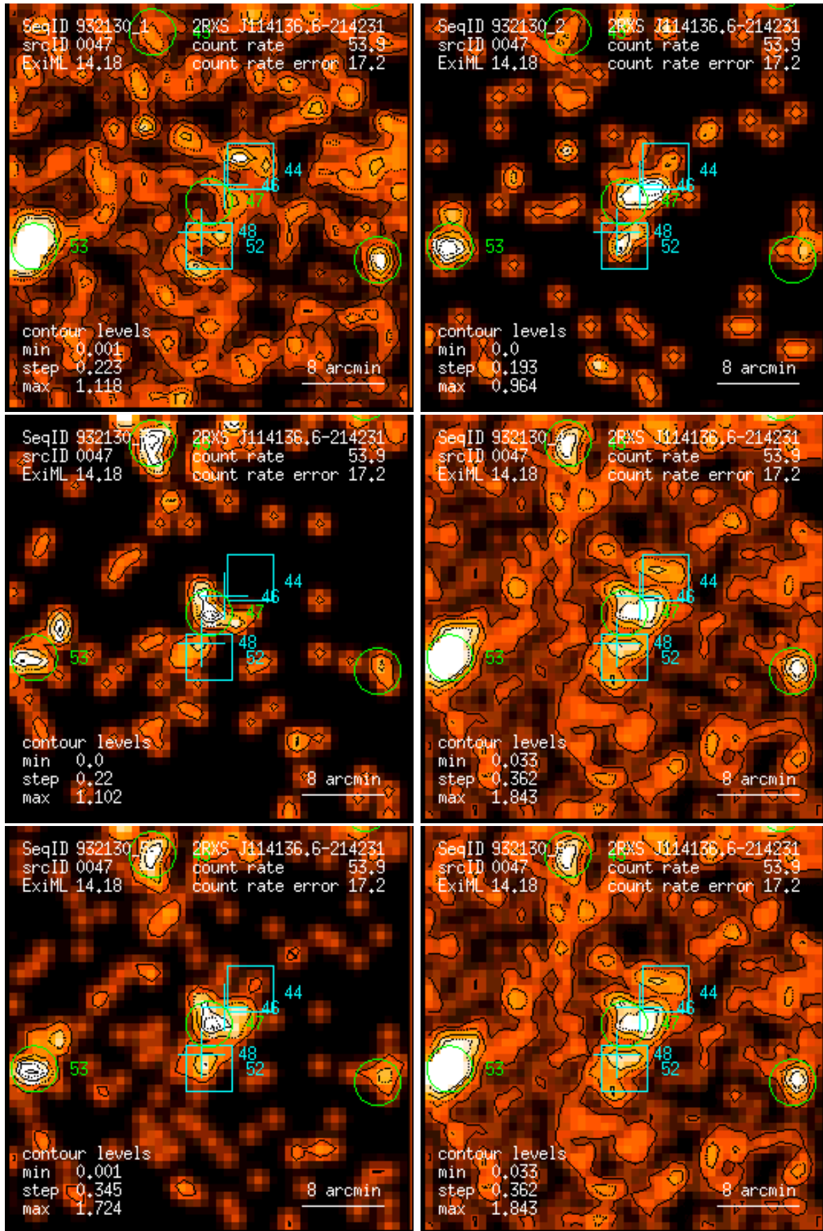
Figure 47: RASS 932130: detection 0047: band rate images, Gaussian filter: (1) PSPC channels 11 – 41, (2) 52 – 90, (3) 91 – 201, (4) 11 – 235, (5) 52 – 201, (6) 11 – 201. Broad band rates in counts/ks. Band rate contour levels in counts/ks/arcmin 2 .
