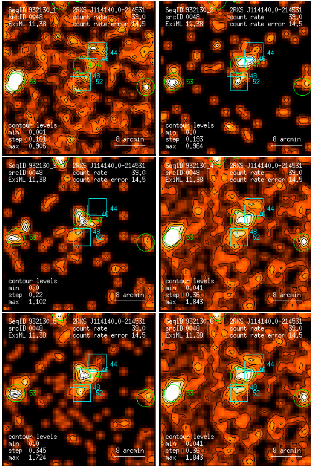
Figure 48: RASS 932130: detection 0048: band rate images, Gaussian filter: (1) PSPC channels 11 – 41, (2) 52 – 90, (3) 91 – 201, (4) 11 – 235, (5) 52 – 201, (6) 11 – 201. Broad band rates in counts/ks. Band rate contour levels in counts/ks/arcmin 2 .
