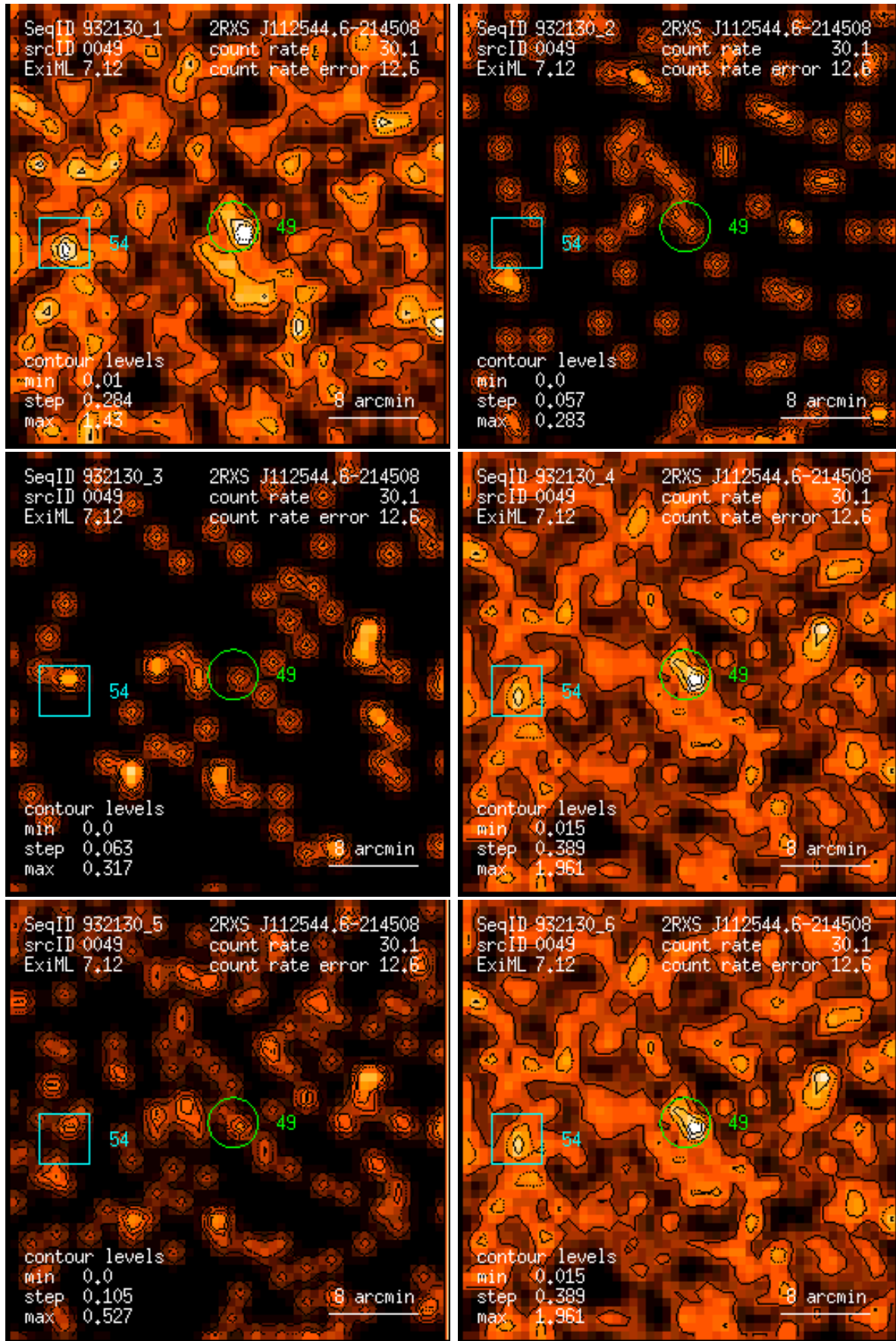
Figure 49: RASS 932130: detection 0049: band rate images, Gaussian filter: (1) PSPC channels 11 – 41, (2) 52 – 90, (3) 91 – 201, (4) 11 – 235, (5) 52 – 201, (6) 11 – 201. Broad band rates in counts/ks. Band rate contour levels in counts/ks/arcmin 2 .
