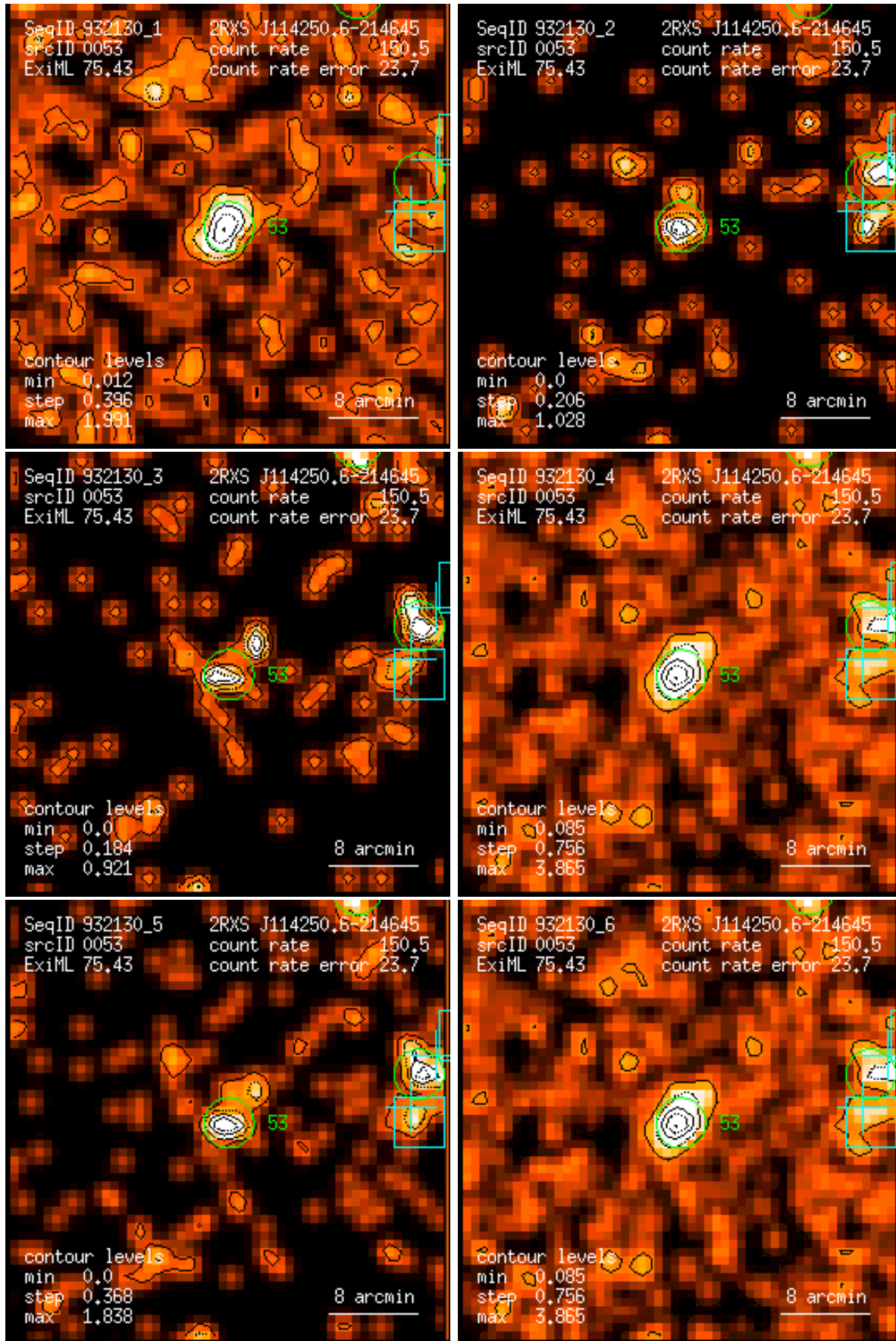
Figure 53: RASS 932130: detection 0053: band rate images, Gaussian filter: (1) PSPC channels 11 – 41, (2) 52 – 90, (3) 91 – 201, (4) 11 – 235, (5) 52 – 201, (6) 11 – 201. Broad band rates in counts/ks. Band rate contour levels in counts/ks/arcmin 2 .
