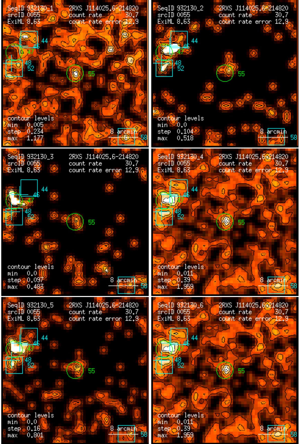
Figure 55: RASS 932130: detection 0055: band rate images, Gaussian filter: (1) PSPC channels 11 – 41, (2) 52 – 90, (3) 91 – 201, (4) 11 – 235, (5) 52 – 201, (6) 11 – 201. Broad band rates in counts/ks. Band rate contour levels in counts/ks/arcmin 2 .
