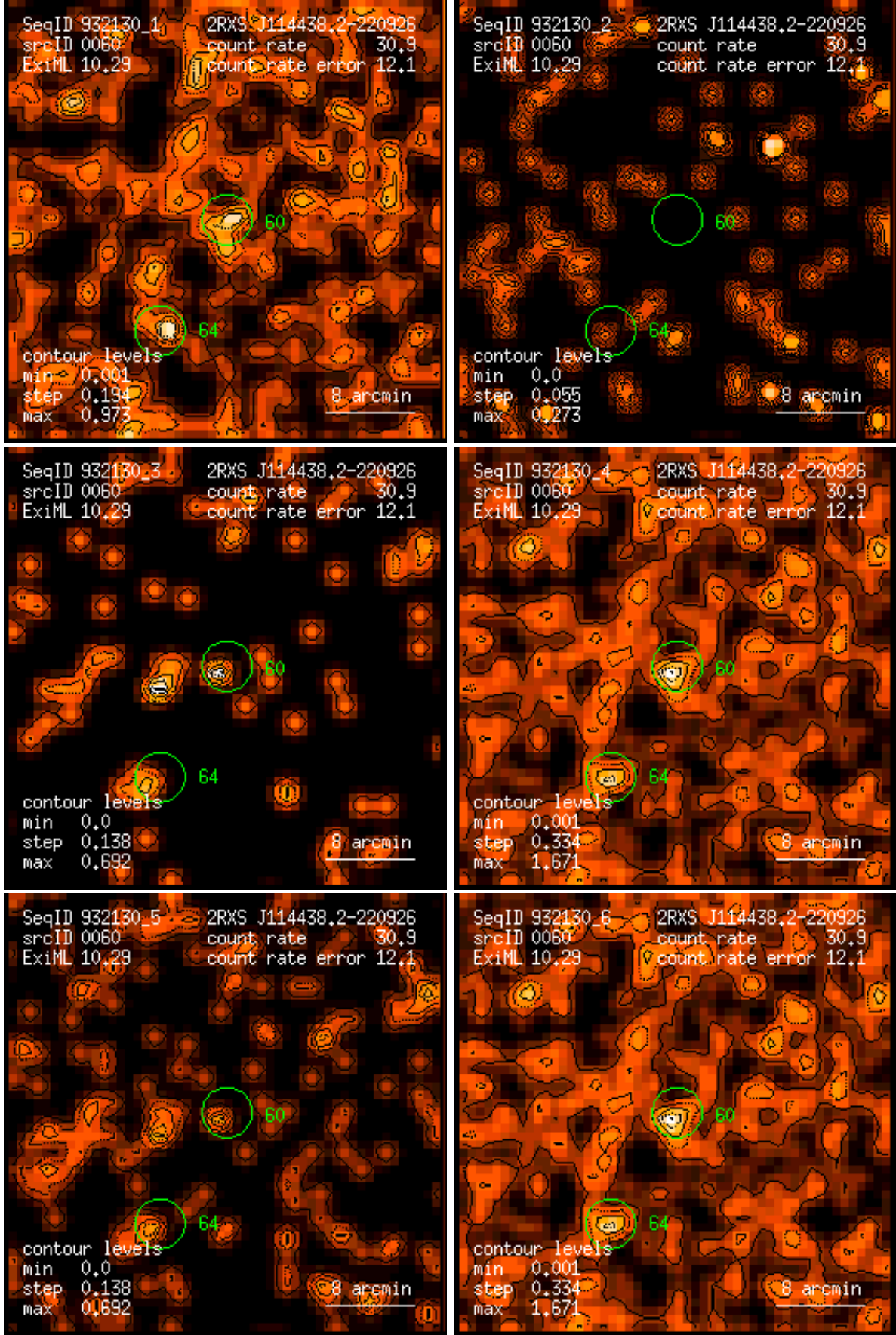
Figure 60: RASS 932130: detection 0060: band rate images, Gaussian filter: (1) PSPC channels 11 – 41, (2) 52 – 90, (3) 91 – 201, (4) 11 – 235, (5) 52 – 201, (6) 11 – 201. Broad band rates in counts/ks. Band rate contour levels in counts/ks/arcmin 2 .
