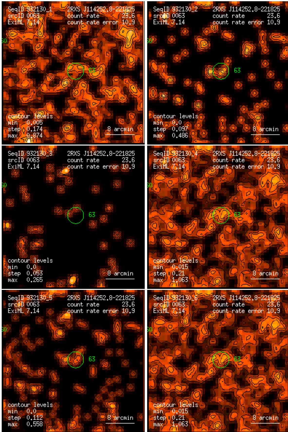
Figure 63: RASS 932130: detection 0063: band rate images, Gaussian filter: (1) PSPC channels 11 – 41, (2) 52 – 90, (3) 91 – 201, (4) 11 – 235, (5) 52 – 201, (6) 11 – 201. Broad band rates in counts/ks. Band rate contour levels in counts/ks/arcmin 2 .
