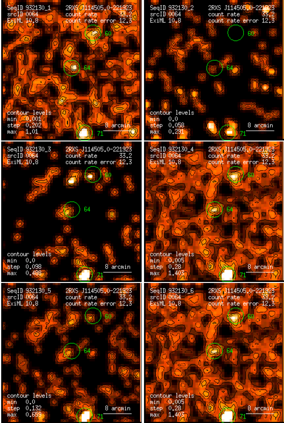
Figure 64: RASS 932130: detection 0064: band rate images, Gaussian filter: (1) PSPC channels 11 – 41, (2) 52 – 90, (3) 91 – 201, (4) 11 – 235, (5) 52 – 201, (6) 11 – 201. Broad band rates in counts/ks. Band rate contour levels in counts/ks/arcmin 2 .
