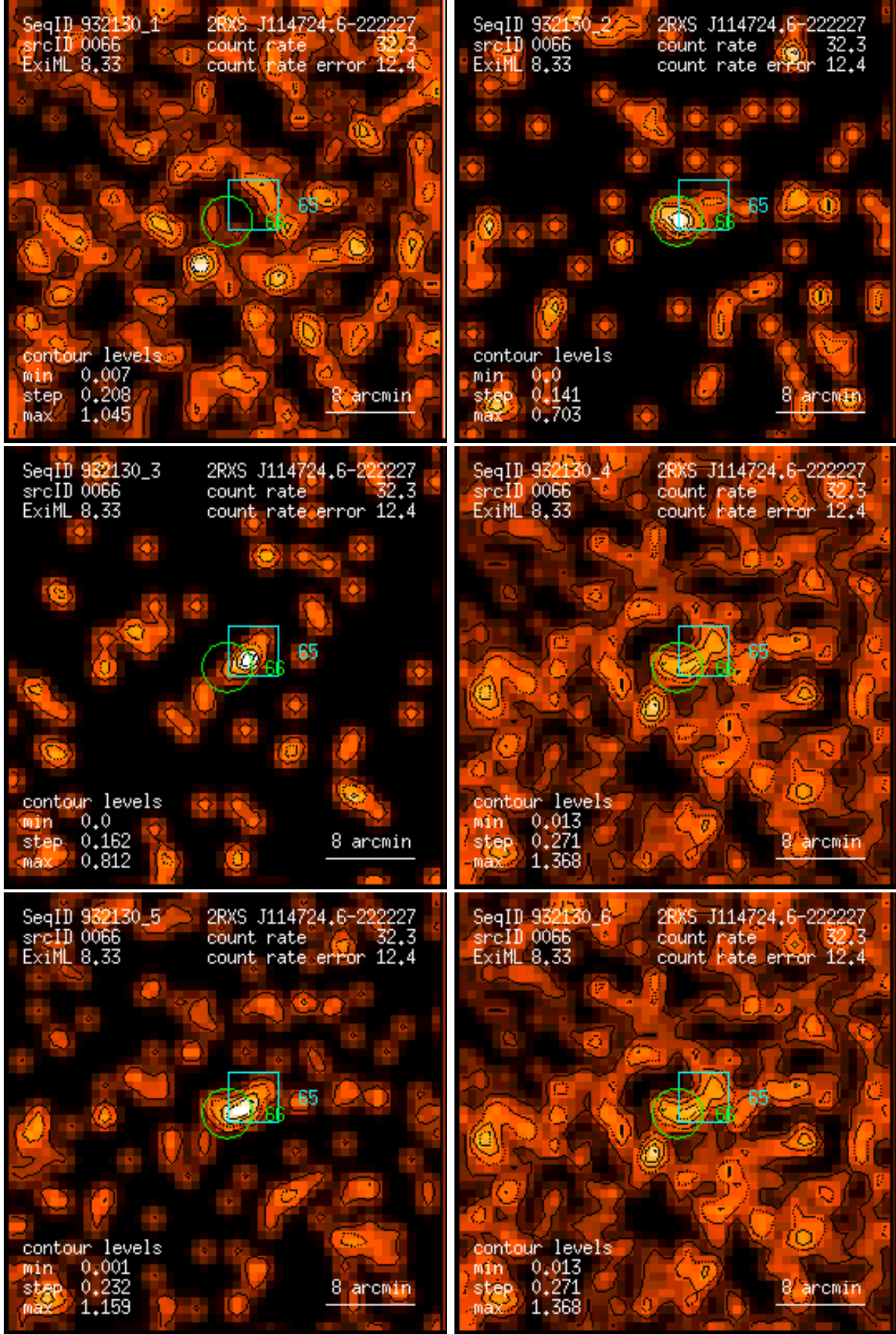
Figure 66: RASS 932130: detection 0066: band rate images, Gaussian filter: (1) PSPC channels 11 – 41, (2) 52 – 90, (3) 91 – 201, (4) 11 – 235, (5) 52 – 201, (6) 11 – 201. Broad band rates in counts/ks. Band rate contour levels in counts/ks/arcmin 2 .
