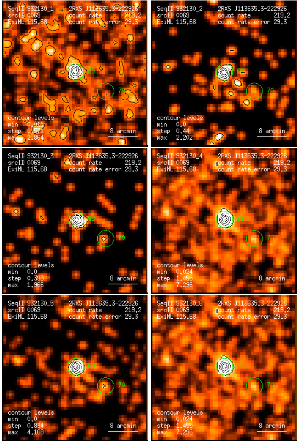
Figure 69: RASS 932130: detection 0069: band rate images, Gaussian filter: (1) PSPC channels 11 – 41, (2) 52 – 90, (3) 91 – 201, (4) 11 – 235, (5) 52 – 201, (6) 11 – 201. Broad band rates in counts/ks. Band rate contour levels in counts/ks/arcmin 2 .
