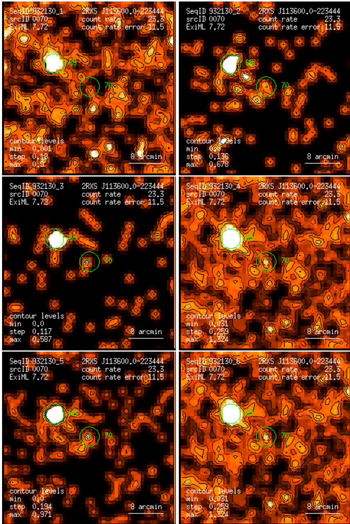
Figure 70: RASS 932130: detection 0070: band rate images, Gaussian filter: (1) PSPC channels 11 – 41, (2) 52 – 90, (3) 91 – 201, (4) 11 – 235, (5) 52 – 201, (6) 11 – 201. Broad band rates in counts/ks. Band rate contour levels in counts/ks/arcmin 2 .
