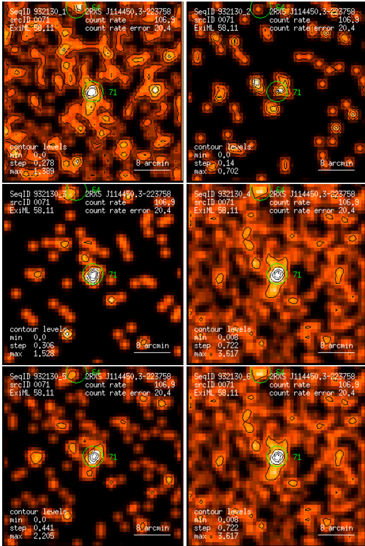
Figure 71: RASS 932130: detection 0071: band rate images, Gaussian filter: (1) PSPC channels 11 – 41, (2) 52 – 90, (3) 91 – 201, (4) 11 – 235, (5) 52 – 201, (6) 11 – 201. Broad band rates in counts/ks. Band rate contour levels in counts/ks/arcmin 2 .
