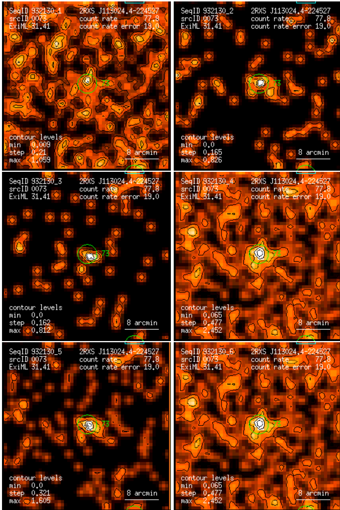
Figure 73: RASS 932130: detection 0073: band rate images, Gaussian filter: (1) PSPC channels 11 – 41, (2) 52 – 90, (3) 91 – 201, (4) 11 – 235, (5) 52 – 201, (6) 11 – 201. Broad band rates in counts/ks. Band rate contour levels in counts/ks/arcmin 2 .
