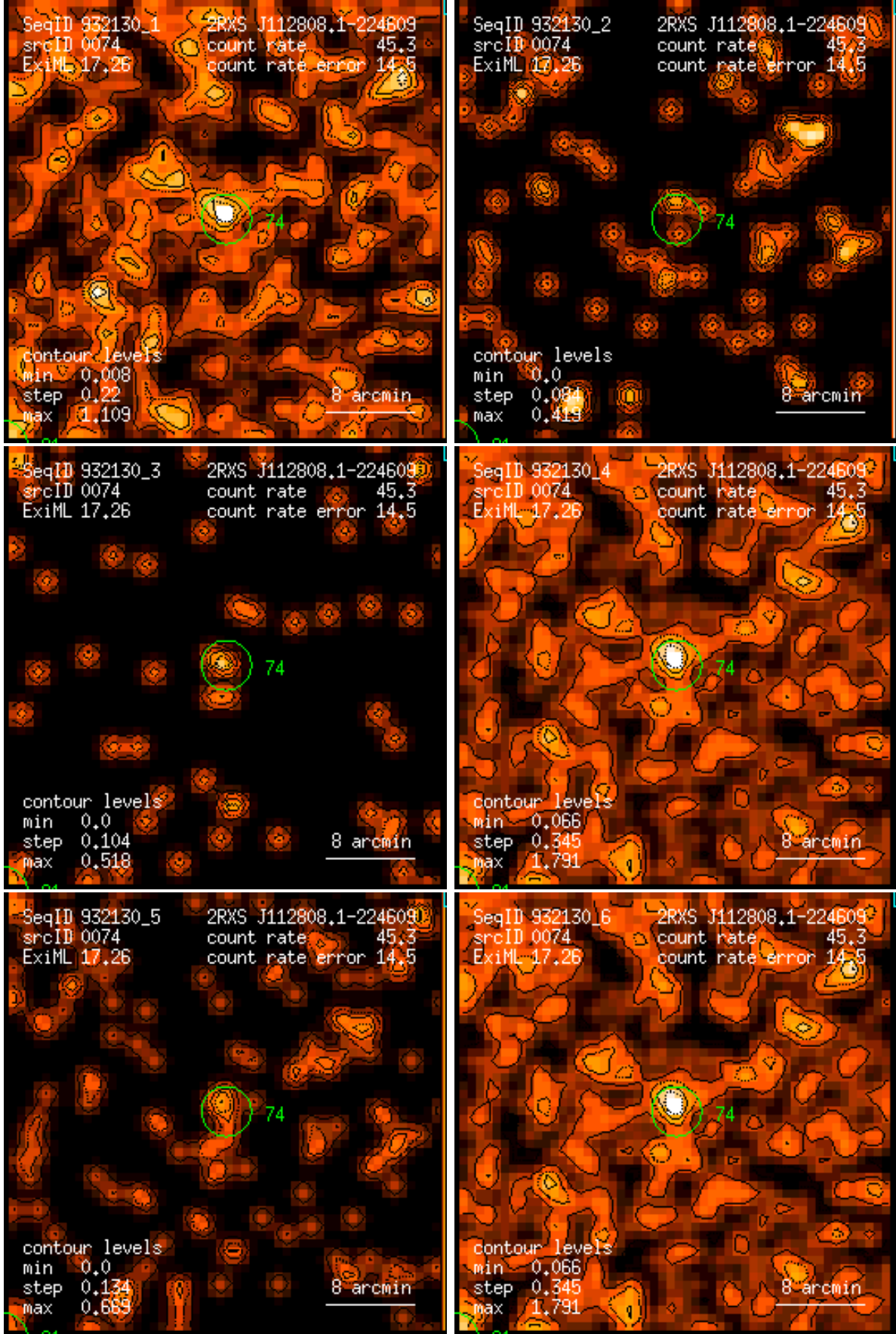
Figure 74: RASS 932130: detection 0074: band rate images, Gaussian filter: (1) PSPC channels 11 – 41, (2) 52 – 90, (3) 91 – 201, (4) 11 – 235, (5) 52 – 201, (6) 11 – 201. Broad band rates in counts/ks. Band rate contour levels in counts/ks/arcmin 2 .
