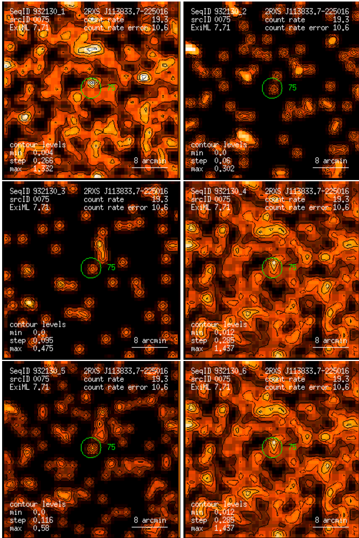
Figure 75: RASS 932130: detection 0075: band rate images, Gaussian filter: (1) PSPC channels 11 – 41, (2) 52 – 90, (3) 91 – 201, (4) 11 – 235, (5) 52 – 201, (6) 11 – 201. Broad band rates in counts/ks. Band rate contour levels in counts/ks/arcmin 2 .
