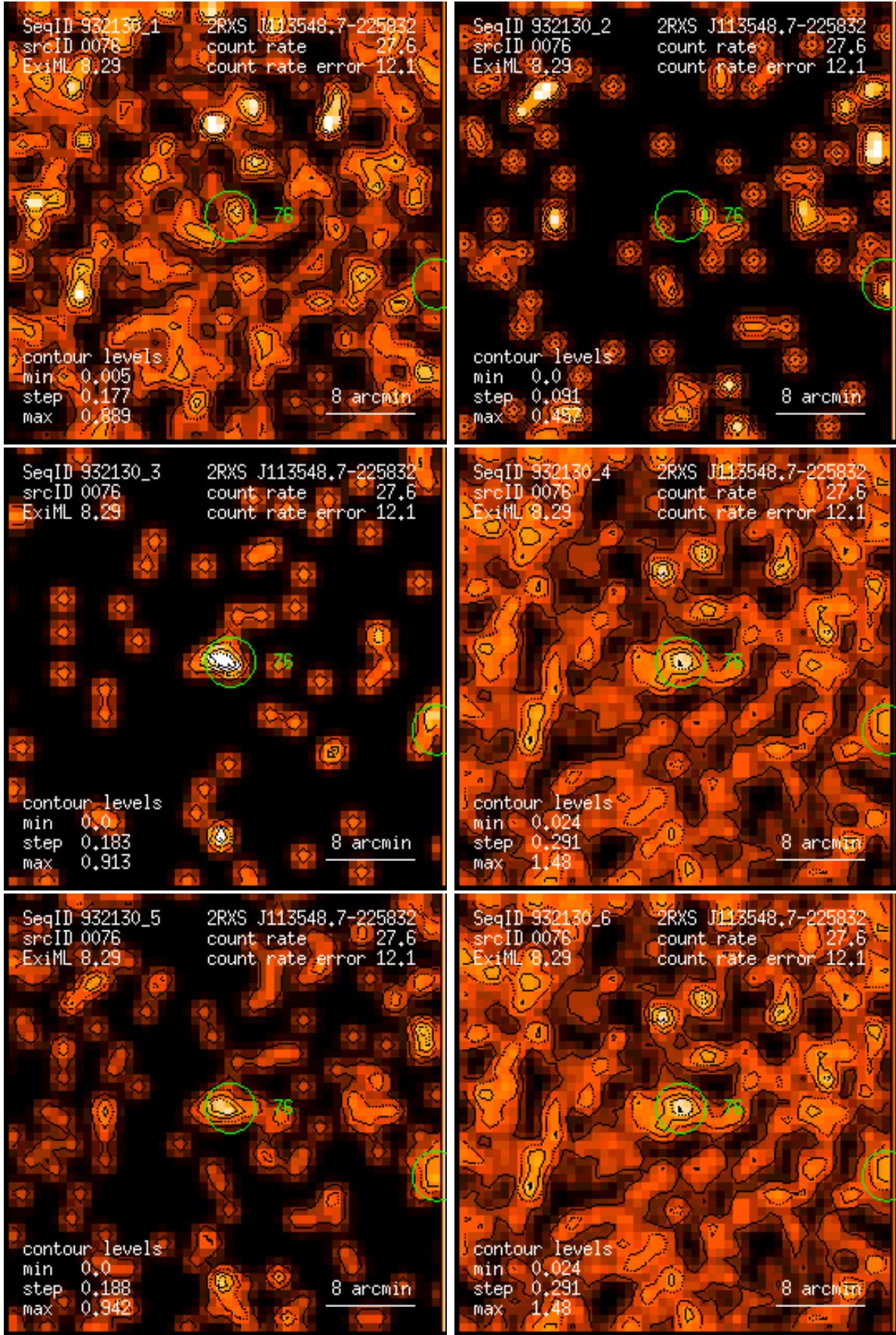
Figure 76: RASS 932130: detection 0076: band rate images, Gaussian filter: (1) PSPC channels 11 – 41, (2) 52 – 90, (3) 91 – 201, (4) 11 – 235, (5) 52 – 201, (6) 11 – 201. Broad band rates in counts/ks. Band rate contour levels in counts/ks/arcmin 2 .
