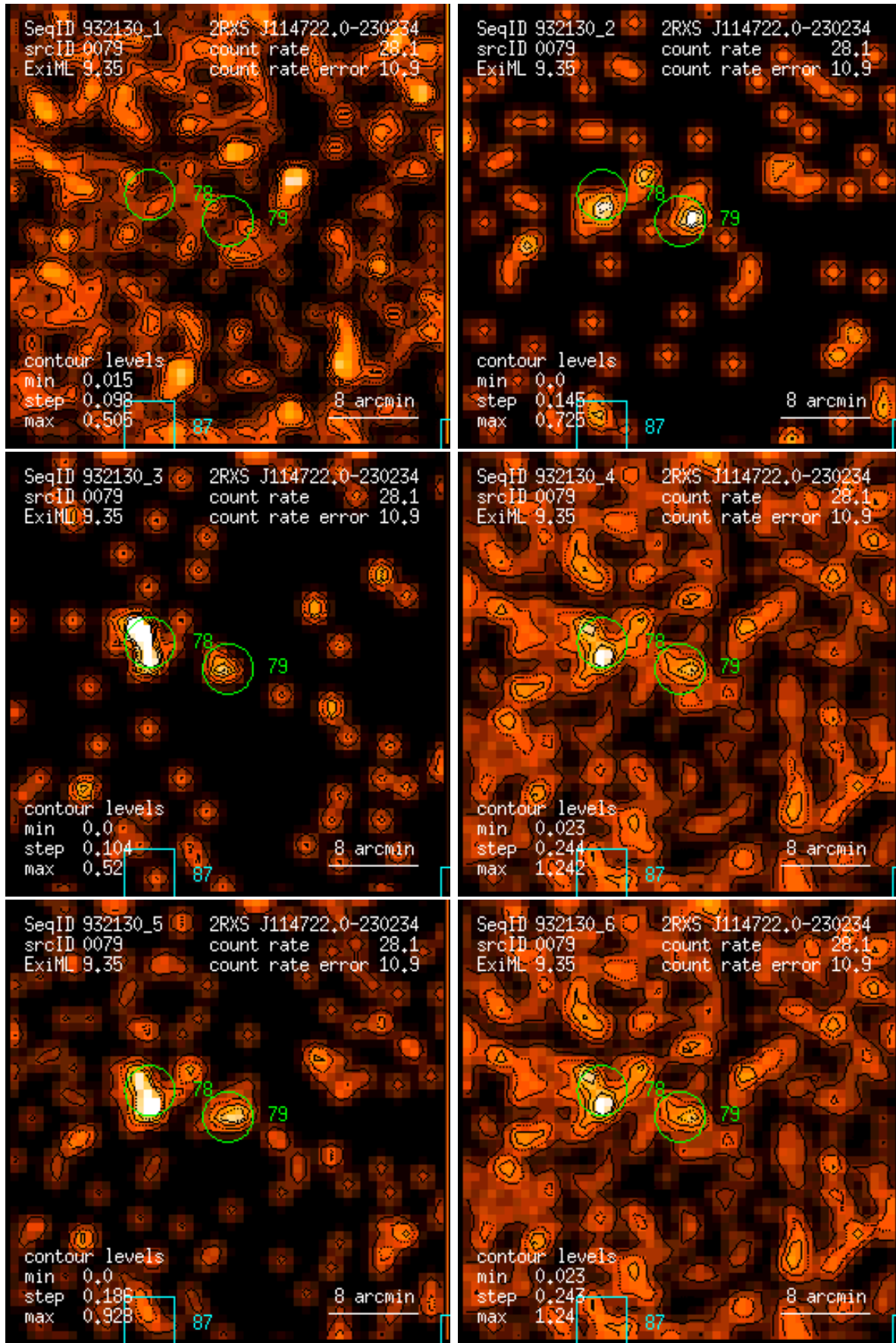
Figure 79: RASS 932130: detection 0079: band rate images, Gaussian filter: (1) PSPC channels 11 – 41, (2) 52 – 90, (3) 91 – 201, (4) 11 – 235, (5) 52 – 201, (6) 11 – 201. Broad band rates in counts/ks. Band rate contour levels in counts/ks/arcmin 2 .
