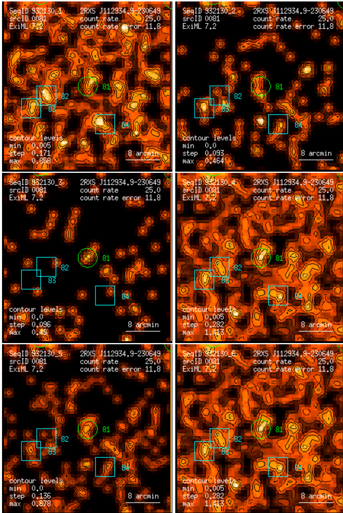
Figure 81: RASS 932130: detection 0081: band rate images, Gaussian filter: (1) PSPC channels 11 – 41, (2) 52 – 90, (3) 91 – 201, (4) 11 – 235, (5) 52 – 201, (6) 11 – 201. Broad band rates in counts/ks. Band rate contour levels in counts/ks/arcmin 2 .
