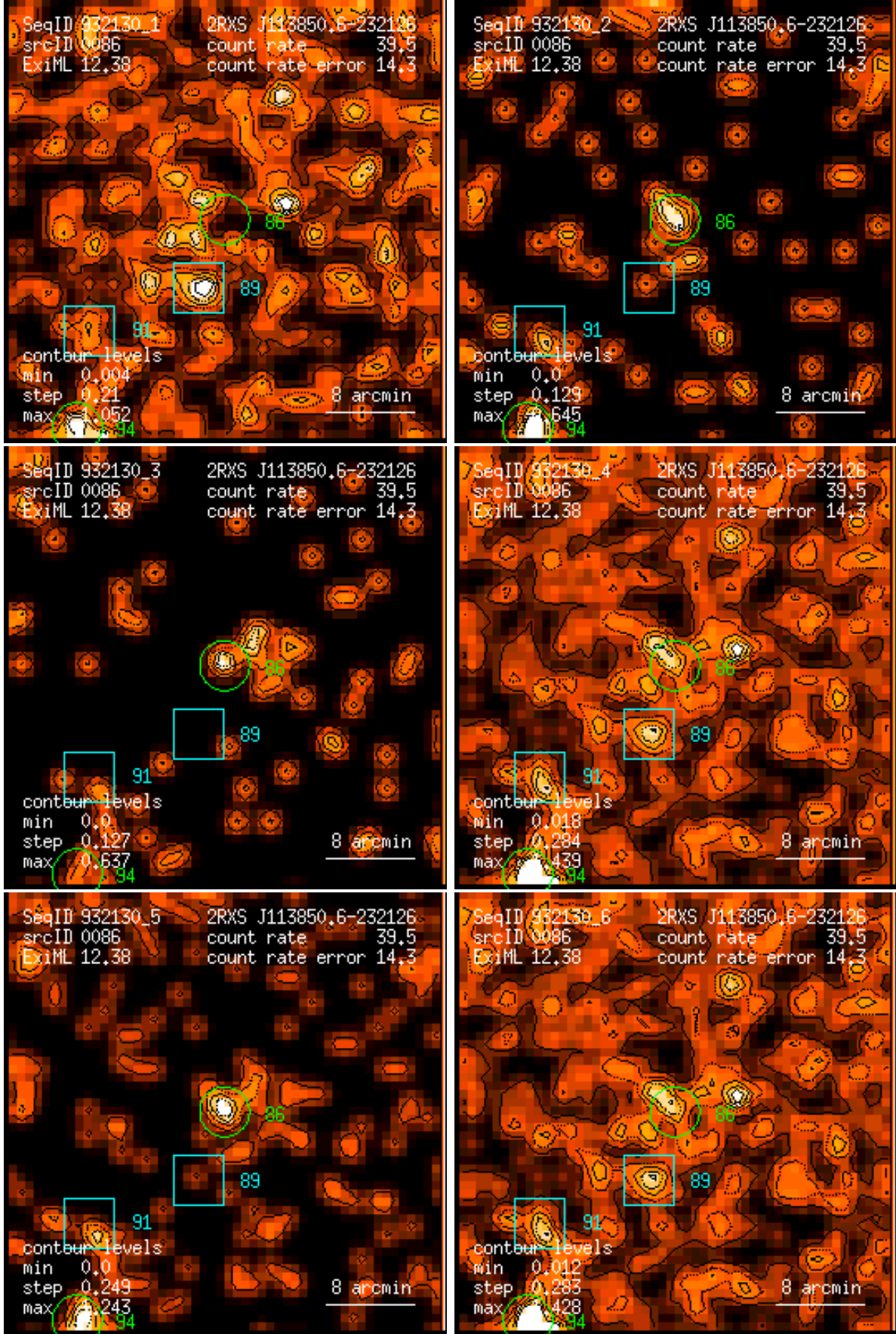
Figure 86: RASS 932130: detection 0086: band rate images, Gaussian filter: (1) PSPC channels 11 – 41, (2) 52 – 90, (3) 91 – 201, (4) 11 – 235, (5) 52 – 201, (6) 11 – 201. Broad band rates in counts/ks. Band rate contour levels in counts/ks/arcmin 2 .
