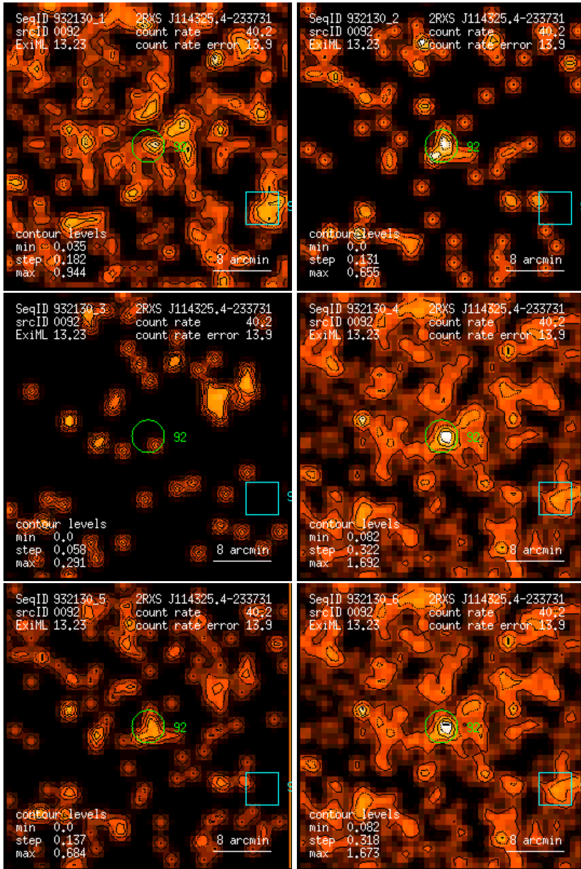
Figure 92: RASS 932130: detection 0092: band rate images, Gaussian filter: (1) PSPC channels 11 – 41, (2) 52 – 90, (3) 91 – 201, (4) 11 – 235, (5) 52 – 201, (6) 11 – 201. Broad band rates in counts/ks. Band rate contour levels in counts/ks/arcmin 2 .
