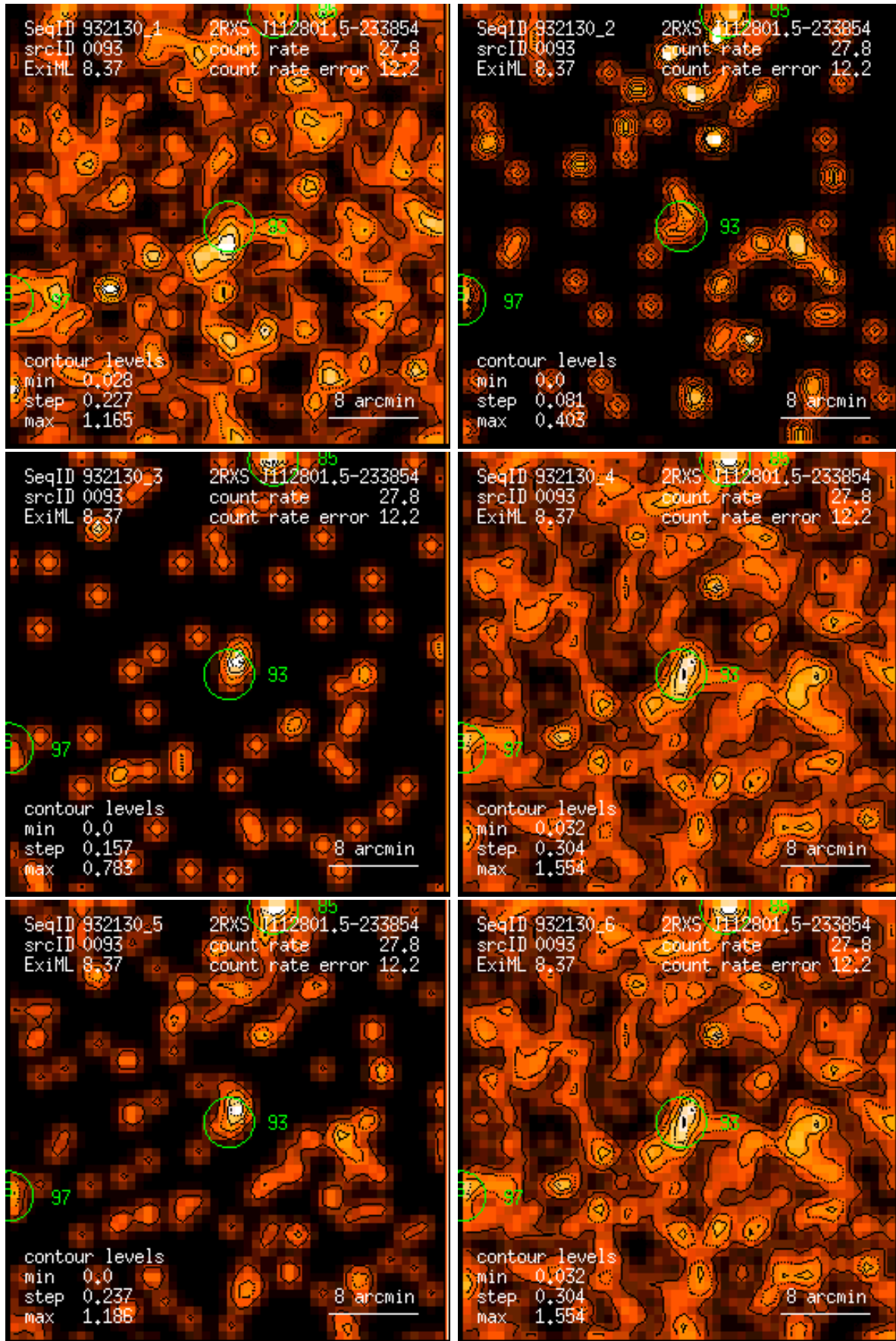
Figure 93: RASS 932130: detection 0093: band rate images, Gaussian filter: (1) PSPC channels 11 – 41, (2) 52 – 90, (3) 91 – 201, (4) 11 – 235, (5) 52 – 201, (6) 11 – 201. Broad band rates in counts/ks. Band rate contour levels in counts/ks/arcmin 2 .
