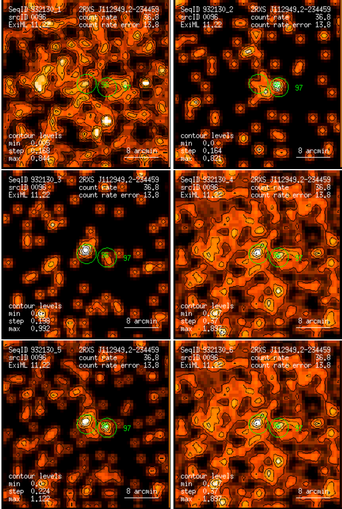
Figure 96: RASS 932130: detection 0096: band rate images, Gaussian filter: (1) PSPC channels 11 – 41, (2) 52 – 90, (3) 91 – 201, (4) 11 – 235, (5) 52 – 201, (6) 11 – 201. Broad band rates in counts/ks. Band rate contour levels in counts/ks/arcmin 2 .
