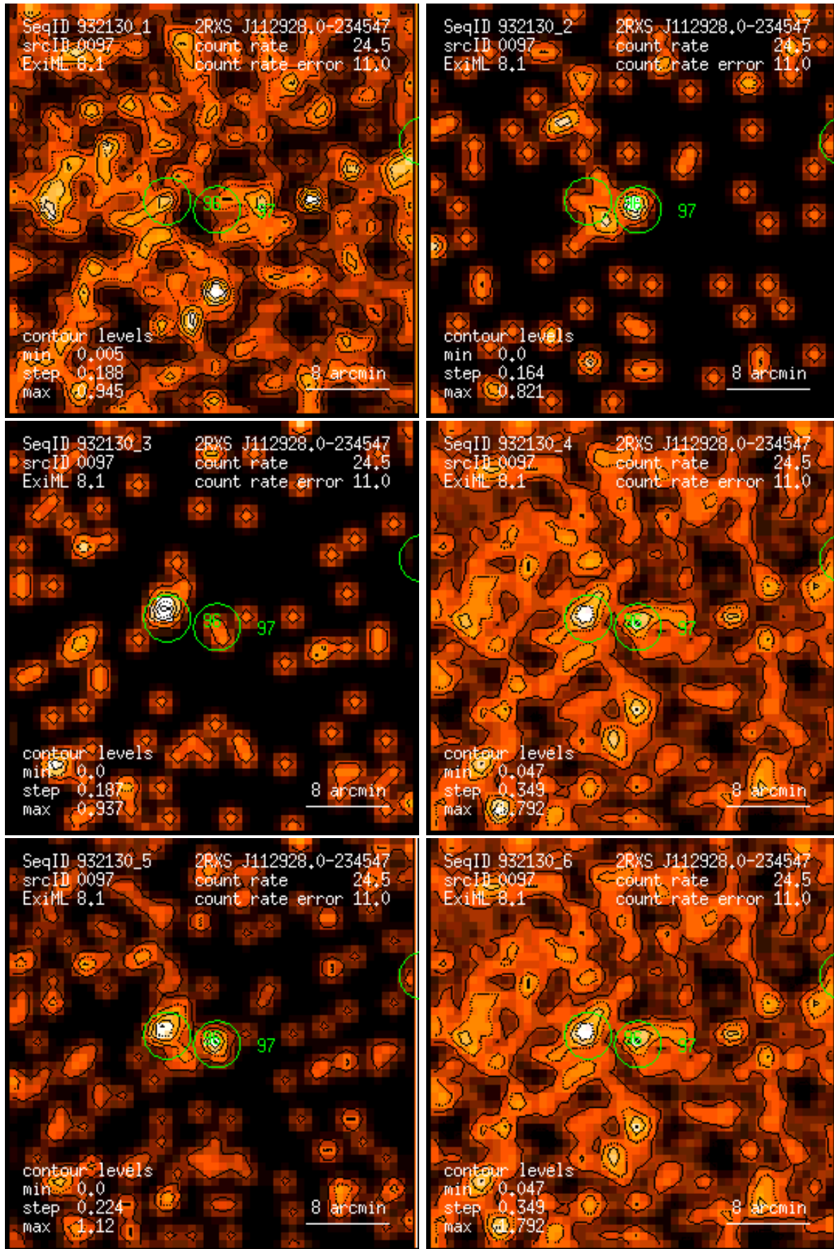
Figure 97: RASS 932130: detection 0097: band rate images, Gaussian filter: (1) PSPC channels 11 – 41, (2) 52 – 90, (3) 91 – 201, (4) 11 – 235, (5) 52 – 201, (6) 11 – 201. Broad band rates in counts/ks. Band rate contour levels in counts/ks/arcmin 2 .
