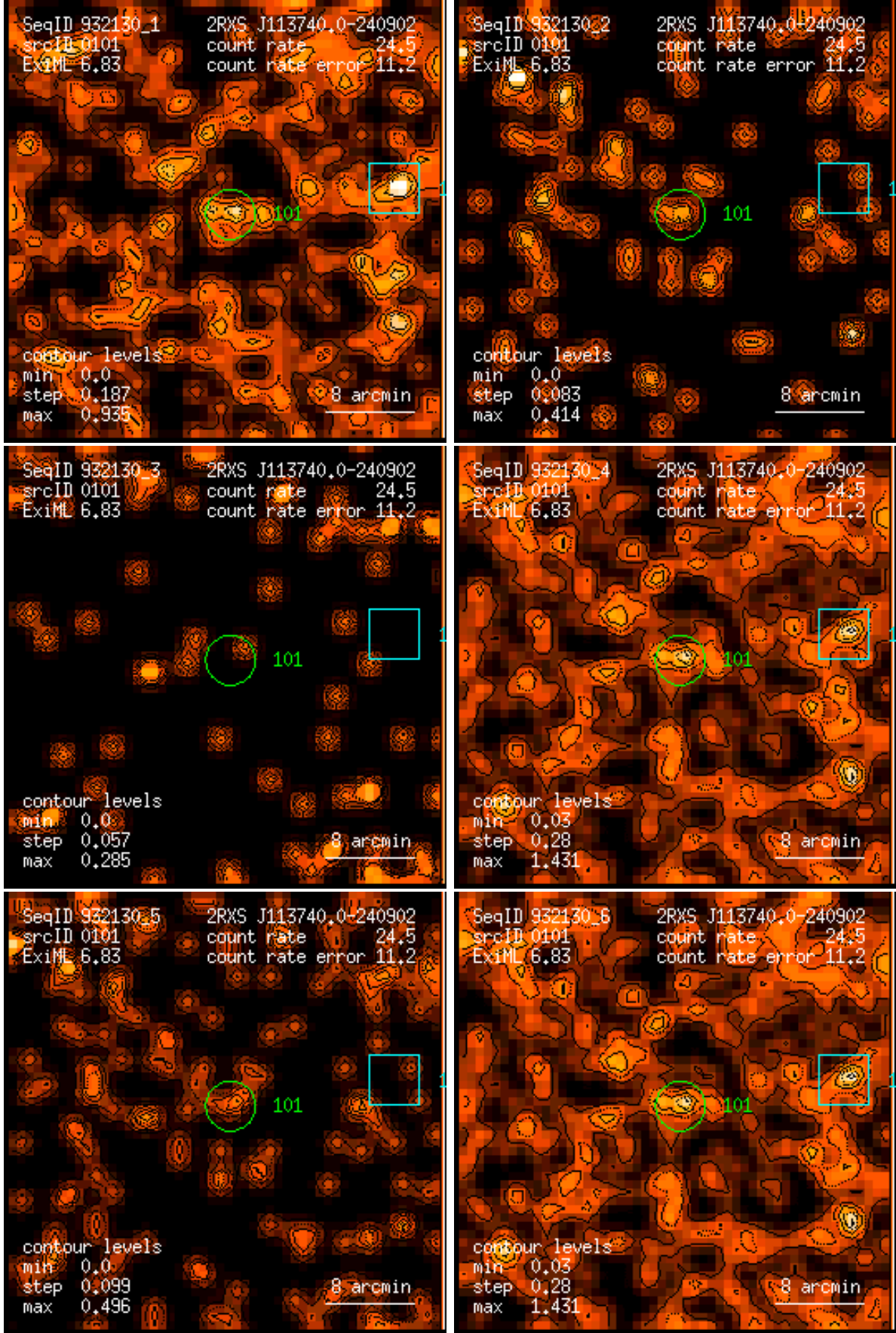
Figure 101: RASS 932130: detection 0101: band rate images, Gaussian filter: (1) PSPC channels 11 – 41, (2) 52 – 90, (3) 91 – 201, (4) 11 – 235, (5) 52 – 201, (6) 11 – 201. Broad band rates in counts/ks. Band rate contour levels in counts/ks/arcmin 2 .
