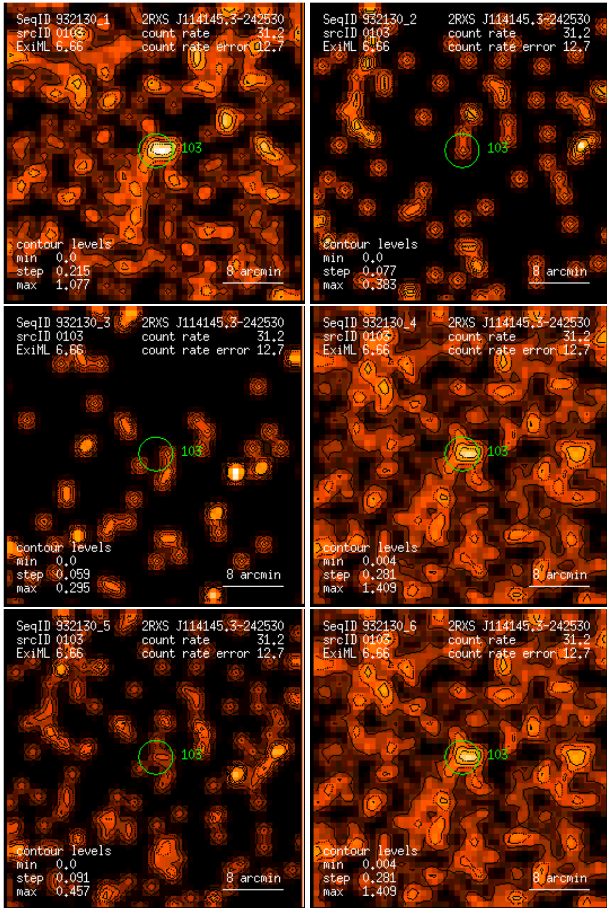
Figure 103: RASS 932130: detection 0103: band rate images, Gaussian filter: (1) PSPC channels 11 – 41, (2) 52 – 90, (3) 91 – 201, (4) 11 – 235, (5) 52 – 201, (6) 11 – 201. Broad band rates in counts/ks. Band rate contour levels in counts/ks/arcmin 2 .
