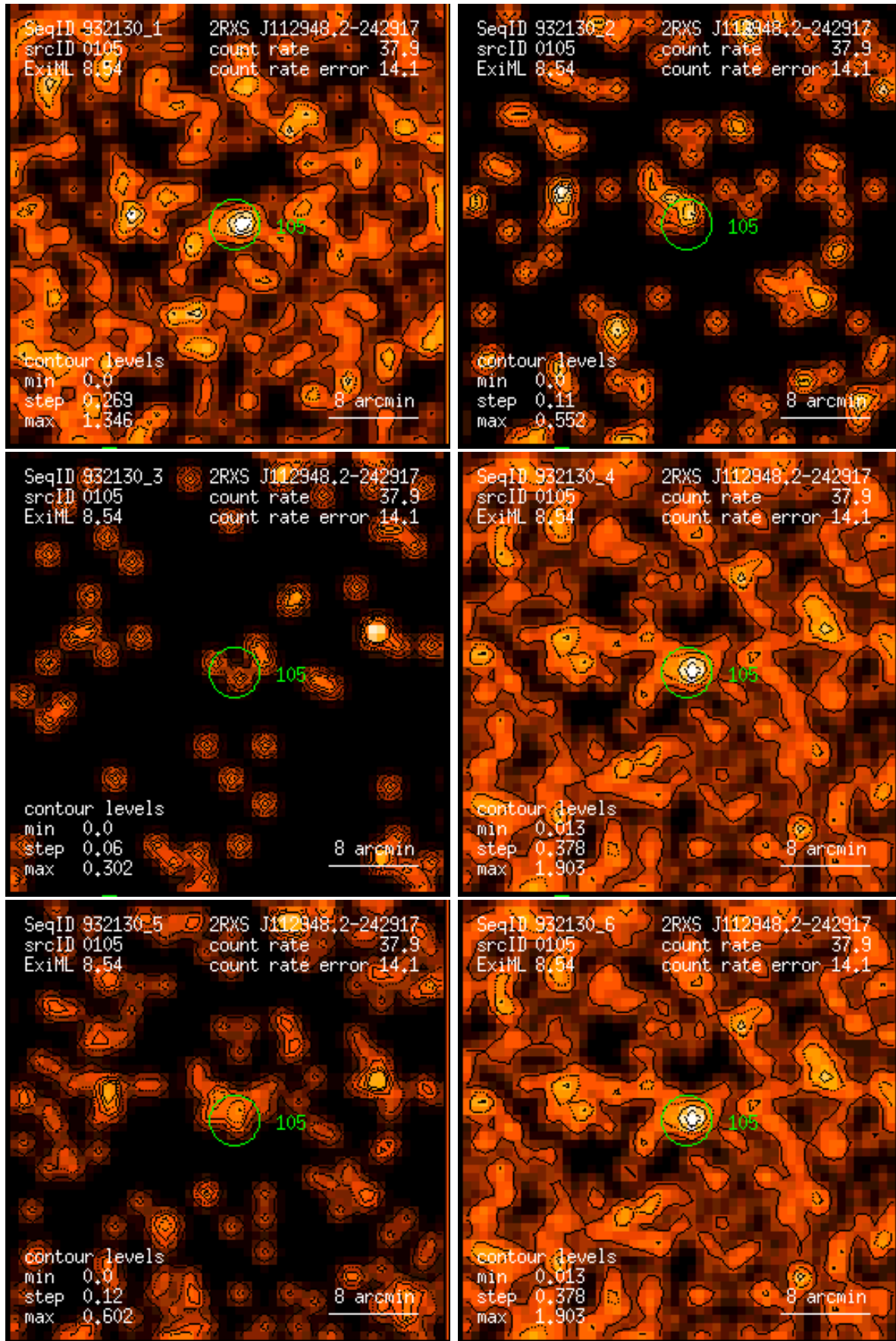
Figure 105: RASS 932130: detection 0105: band rate images, Gaussian filter: (1) PSPC channels 11 – 41, (2) 52 – 90, (3) 91 – 201, (4) 11 – 235, (5) 52 – 201, (6) 11 – 201. Broad band rates in counts/ks. Band rate contour levels in counts/ks/arcmin 2 .
