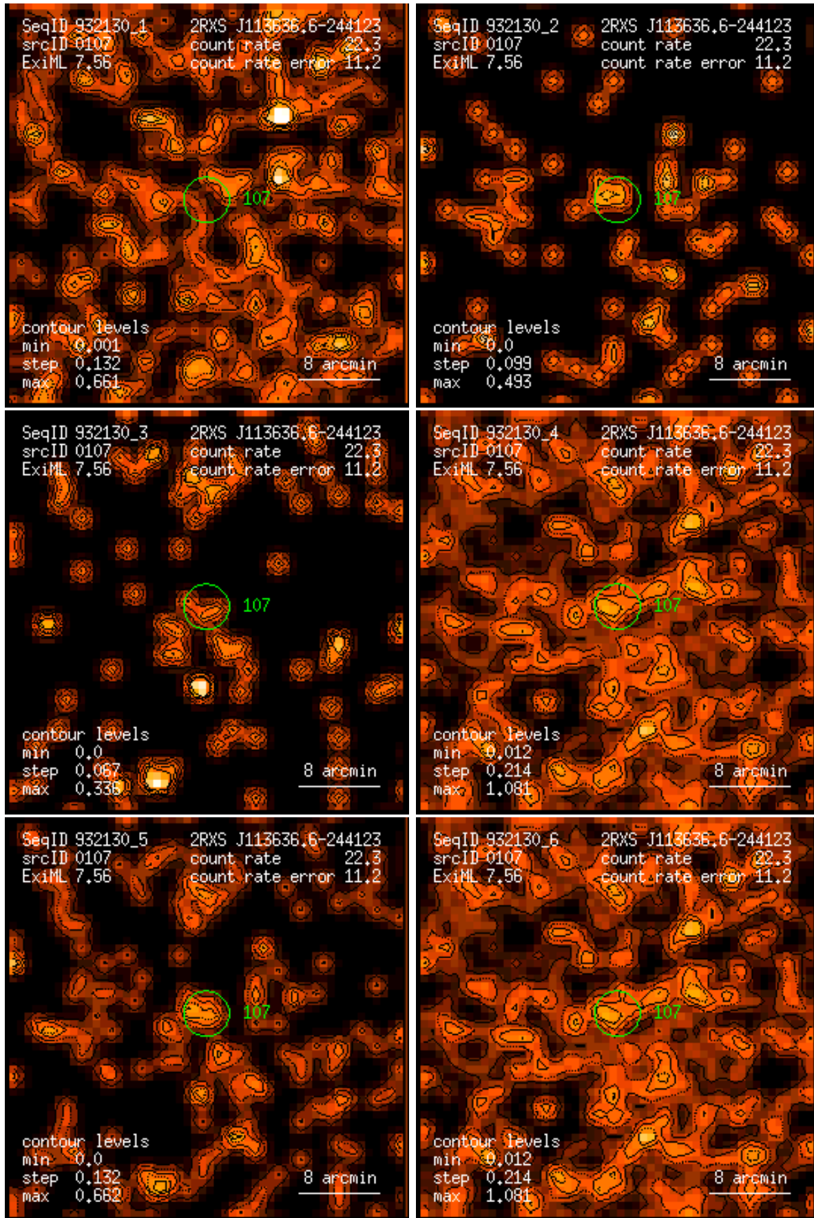
Figure 107: RASS 932130: detection 0107: band rate images, Gaussian filter: (1) PSPC channels 11 – 41, (2) 52 – 90, (3) 91 – 201, (4) 11 – 235, (5) 52 – 201, (6) 11 – 201. Broad band rates in counts/ks. Band rate contour levels in counts/ks/arcmin 2 .
