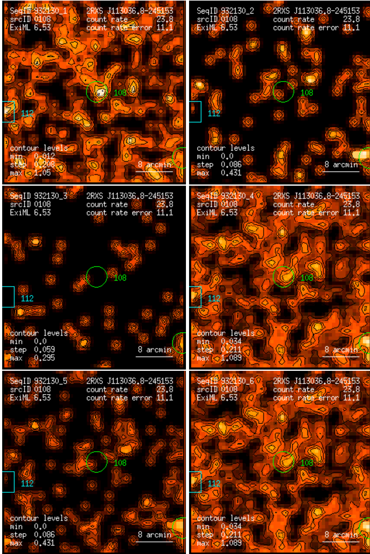
Figure 108: RASS 932130: detection 0108: band rate images, Gaussian filter: (1) PSPC channels 11 – 41, (2) 52 – 90, (3) 91 – 201, (4) 11 – 235, (5) 52 – 201, (6) 11 – 201. Broad band rates in counts/ks. Band rate contour levels in counts/ks/arcmin 2 .
