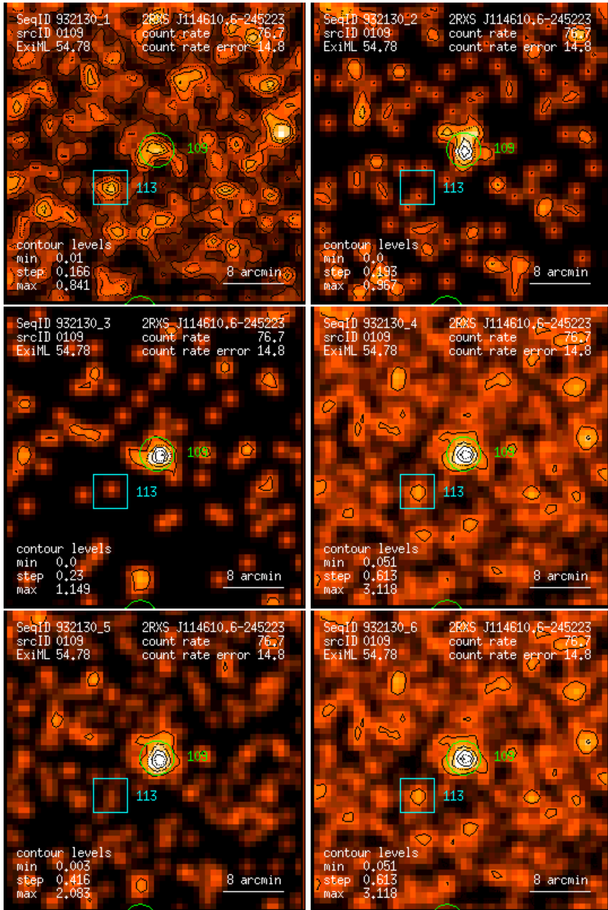
Figure 109: RASS 932130: detection 0109: band rate images, Gaussian filter: (1) PSPC channels 11 – 41, (2) 52 – 90, (3) 91 – 201, (4) 11 – 235, (5) 52 – 201, (6) 11 – 201. Broad band rates in counts/ks. Band rate contour levels in counts/ks/arcmin 2 .
