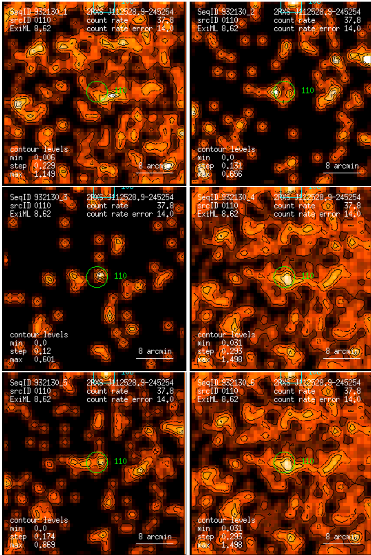
Figure 110: RASS 932130: detection 0110: band rate images, Gaussian filter: (1) PSPC channels 11 – 41, (2) 52 – 90, (3) 91 – 201, (4) 11 – 235, (5) 52 – 201, (6) 11 – 201. Broad band rates in counts/ks. Band rate contour levels in counts/ks/arcmin 2 .
