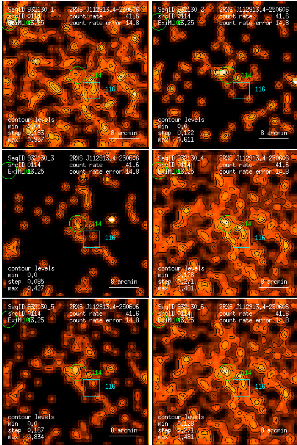
Figure 114: RASS 932130: detection 0114: band rate images, Gaussian filter: (1) PSPC channels 11 – 41, (2) 52 – 90, (3) 91 – 201, (4) 11 – 235, (5) 52 – 201, (6) 11 – 201. Broad band rates in counts/ks. Band rate contour levels in counts/ks/arcmin 2 .
