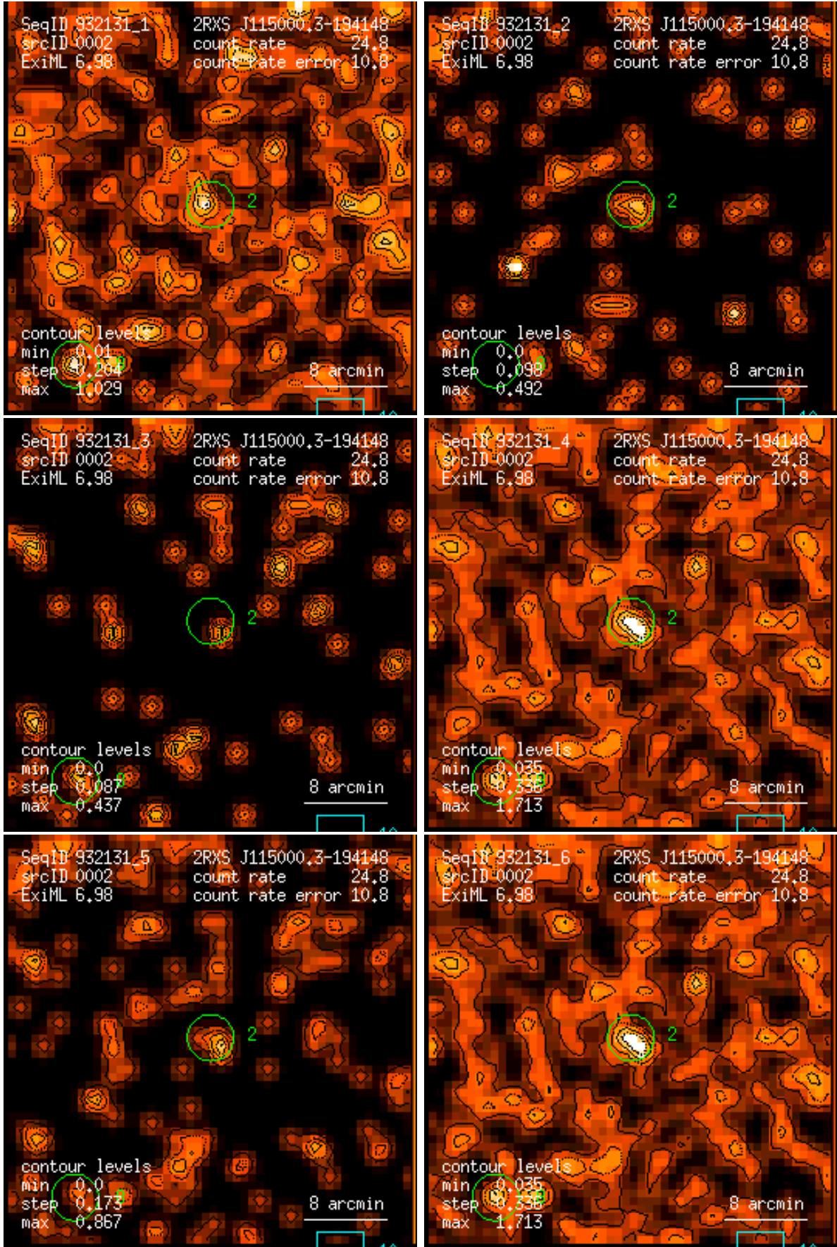
Figure 2: RASS 932131: detection 0002: band rate images, Gaussian filter: (1) PSPC channels 11 – 41, (2) 52 – 90, (3) 91 – 201, (4) 11 – 235, (5) 52 – 201, (6) 11 – 201. Broad band rates in counts/ks. Band rate contour levels in counts/ks/arcmin 2 .
