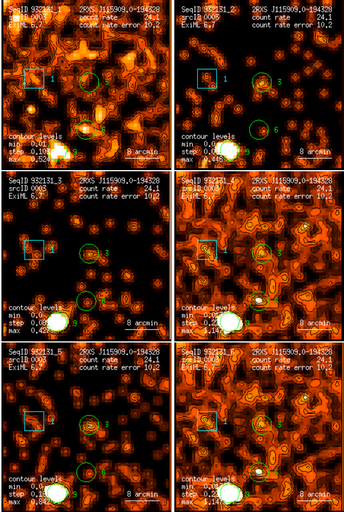
Figure 3: RASS 932131: detection 0003: band rate images, Gaussian filter: (1) PSPC channels 11 – 41, (2) 52 – 90, (3) 91 – 201, (4) 11 – 235, (5) 52 – 201, (6) 11 – 201. Broad band rates in counts/ks. Band rate contour levels in counts/ks/arcmin 2 .
