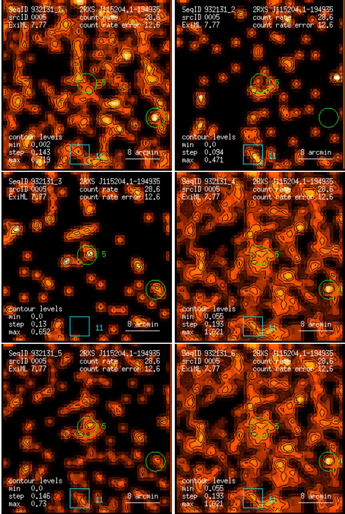
Figure 5: RASS 932131: detection 0005: band rate images, Gaussian filter: (1) PSPC channels 11 – 41, (2) 52 – 90, (3) 91 – 201, (4) 11 – 235, (5) 52 – 201, (6) 11 – 201. Broad band rates in counts/ks. Band rate contour levels in counts/ks/arcmin 2 .
