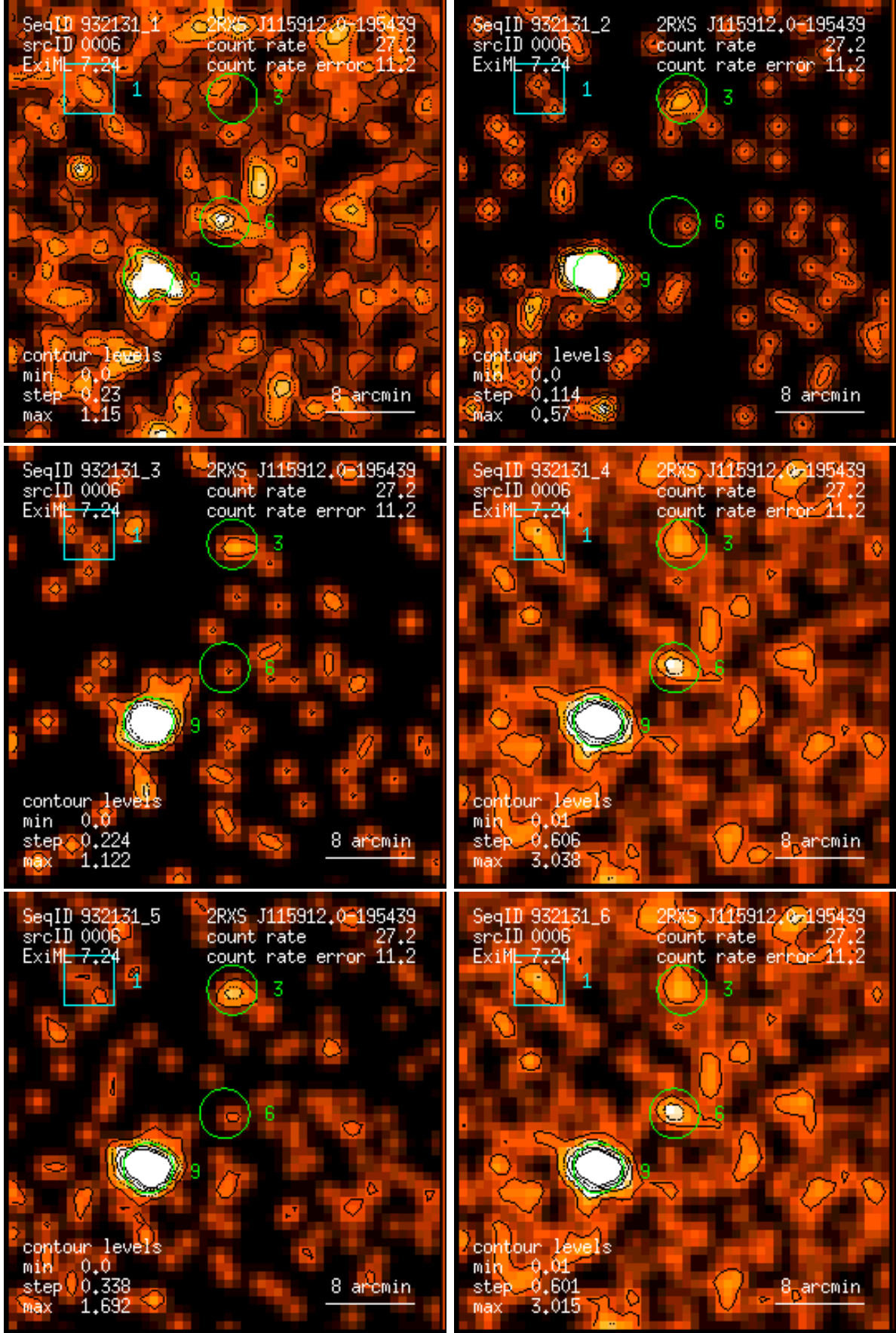
Figure 6: RASS 932131: detection 0006: band rate images, Gaussian filter: (1) PSPC channels 11 – 41, (2) 52 – 90, (3) 91 – 201, (4) 11 – 235, (5) 52 – 201, (6) 11 – 201. Broad band rates in counts/ks. Band rate contour levels in counts/ks/arcmin 2 .
