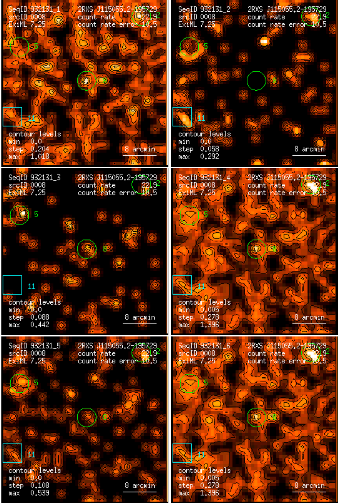
Figure 8: RASS 932131: detection 0008: band rate images, Gaussian filter: (1) PSPC channels 11 – 41, (2) 52 – 90, (3) 91 – 201, (4) 11 – 235, (5) 52 – 201, (6) 11 – 201. Broad band rates in counts/ks. Band rate contour levels in counts/ks/arcmin 2 .
