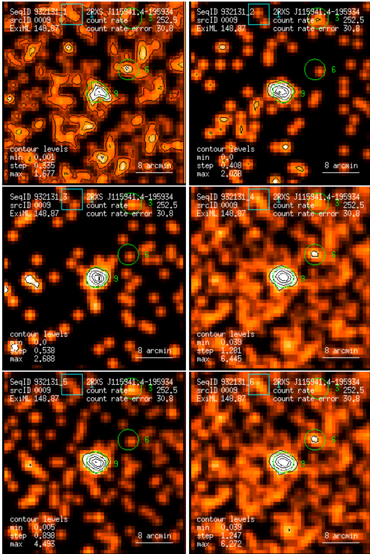
Figure 9: RASS 932131: detection 0009: band rate images, Gaussian filter: (1) PSPC channels 11 – 41, (2) 52 – 90, (3) 91 – 201, (4) 11 – 235, (5) 52 – 201, (6) 11 – 201. Broad band rates in counts/ks. Band rate contour levels in counts/ks/arcmin 2 .
