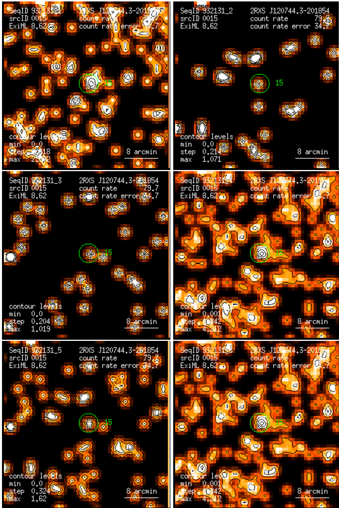
Figure 15: RASS 932131: detection 0015: band rate images, Gaussian filter: (1) PSPC channels 11 – 41, (2) 52 – 90, (3) 91 – 201, (4) 11 – 235, (5) 52 – 201, (6) 11 – 201. Broad band rates in counts/ks. Band rate contour levels in counts/ks/arcmin 2 .
