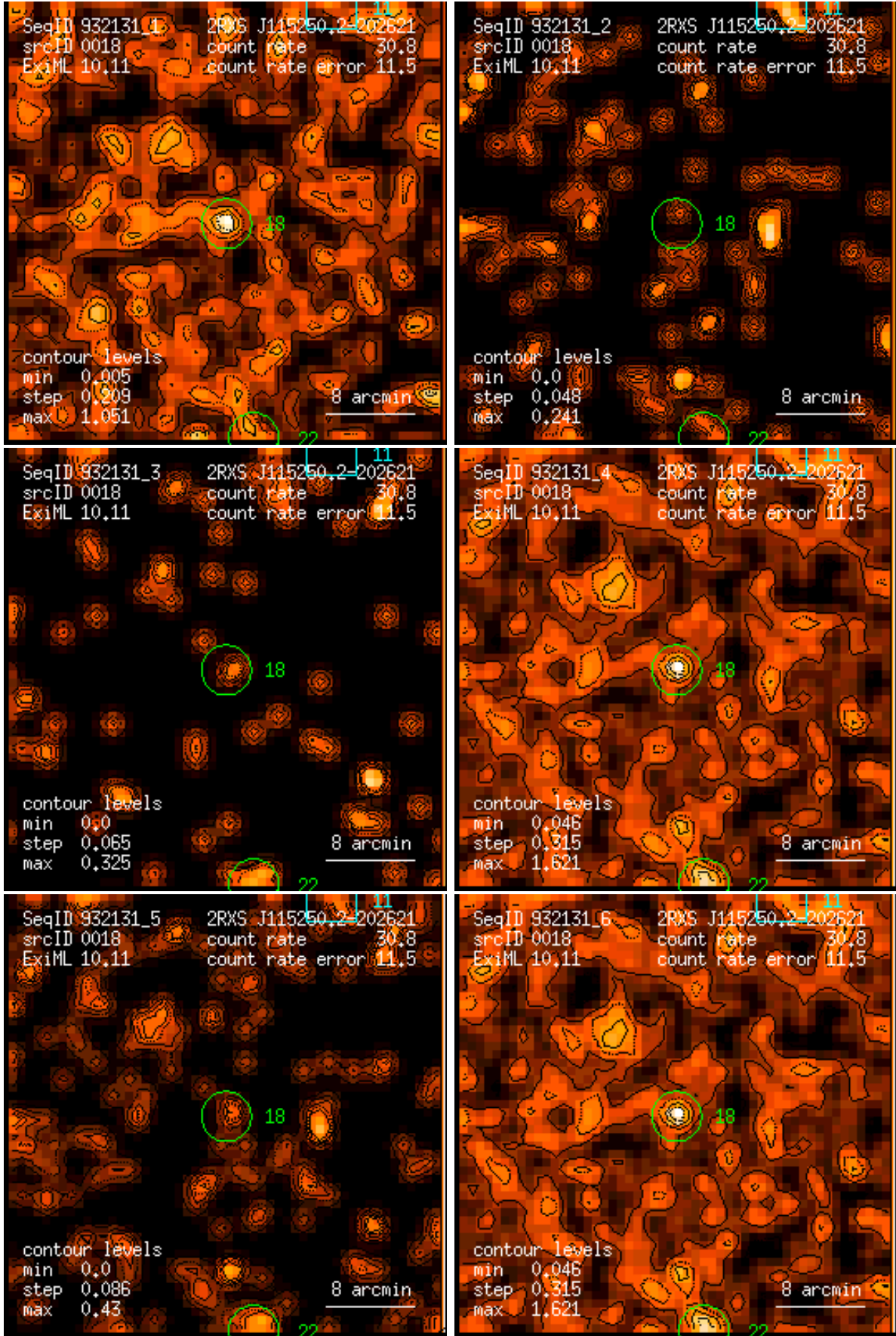
Figure 18: RASS 932131: detection 0018: band rate images, Gaussian filter: (1) PSPC channels 11 – 41, (2) 52 – 90, (3) 91 – 201, (4) 11 – 235, (5) 52 – 201, (6) 11 – 201. Broad band rates in counts/ks. Band rate contour levels in counts/ks/arcmin 2 .
