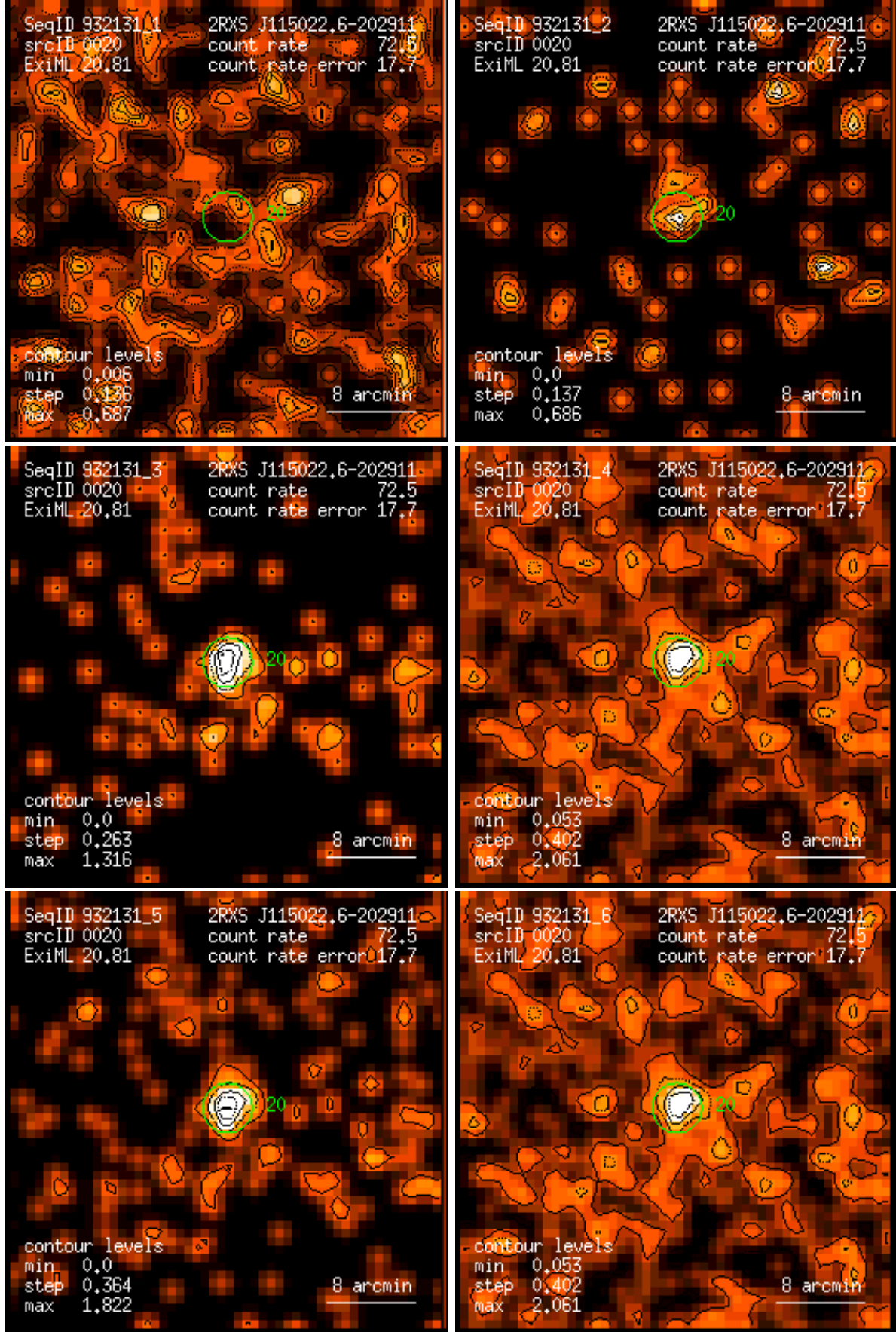
Figure 20: RASS 932131: detection 0020: band rate images, Gaussian filter: (1) PSPC channels 11 – 41, (2) 52 – 90, (3) 91 – 201, (4) 11 – 235, (5) 52 – 201, (6) 11 – 201. Broad band rates in counts/ks. Band rate contour levels in counts/ks/arcmin 2 .
