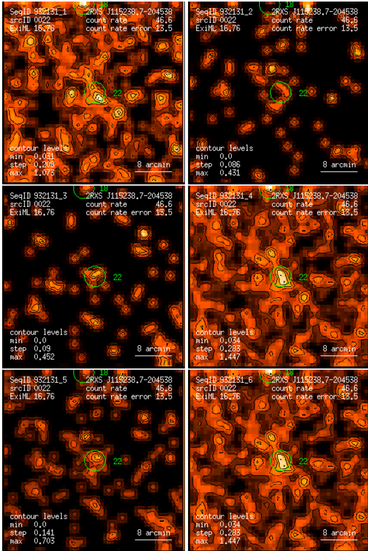
Figure 22: RASS 932131: detection 0022: band rate images, Gaussian filter: (1) PSPC channels 11 – 41, (2) 52 – 90, (3) 91 – 201, (4) 11 – 235, (5) 52 – 201, (6) 11 – 201. Broad band rates in counts/ks. Band rate contour levels in counts/ks/arcmin 2 .
