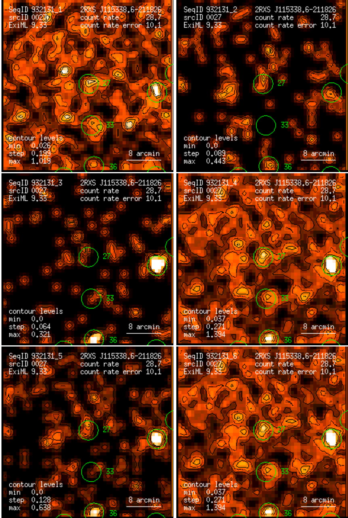
Figure 27: RASS 932131: detection 0027: band rate images, Gaussian filter: (1) PSPC channels 11 – 41, (2) 52 – 90, (3) 91 – 201, (4) 11 – 235, (5) 52 – 201, (6) 11 – 201. Broad band rates in counts/ks. Band rate contour levels in counts/ks/arcmin 2 .
