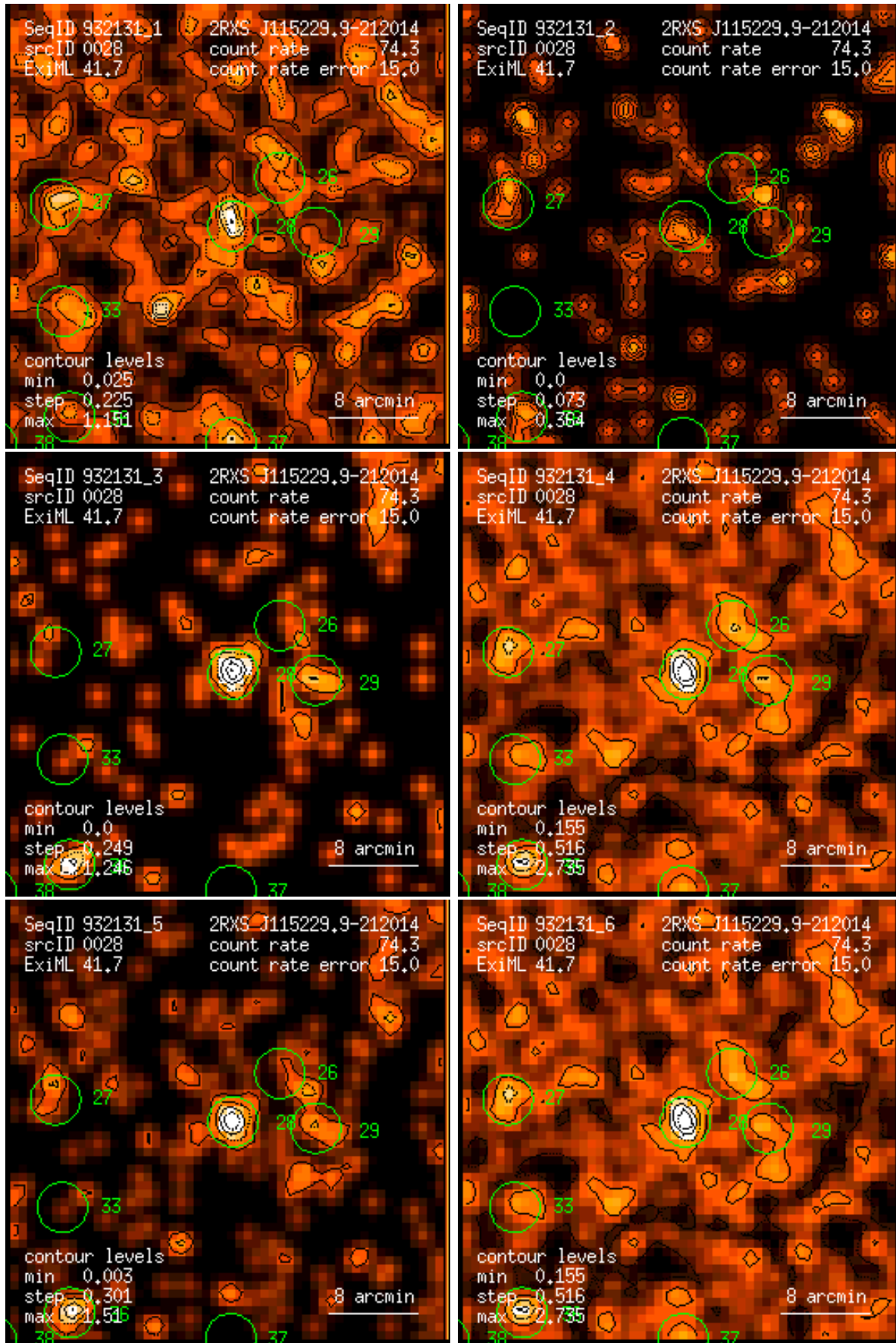
Figure 28: RASS 932131: detection 0028: band rate images, Gaussian filter: (1) PSPC channels 11 – 41, (2) 52 – 90, (3) 91 – 201, (4) 11 – 235, (5) 52 – 201, (6) 11 – 201. Broad band rates in counts/ks. Band rate contour levels in counts/ks/arcmin 2 .
