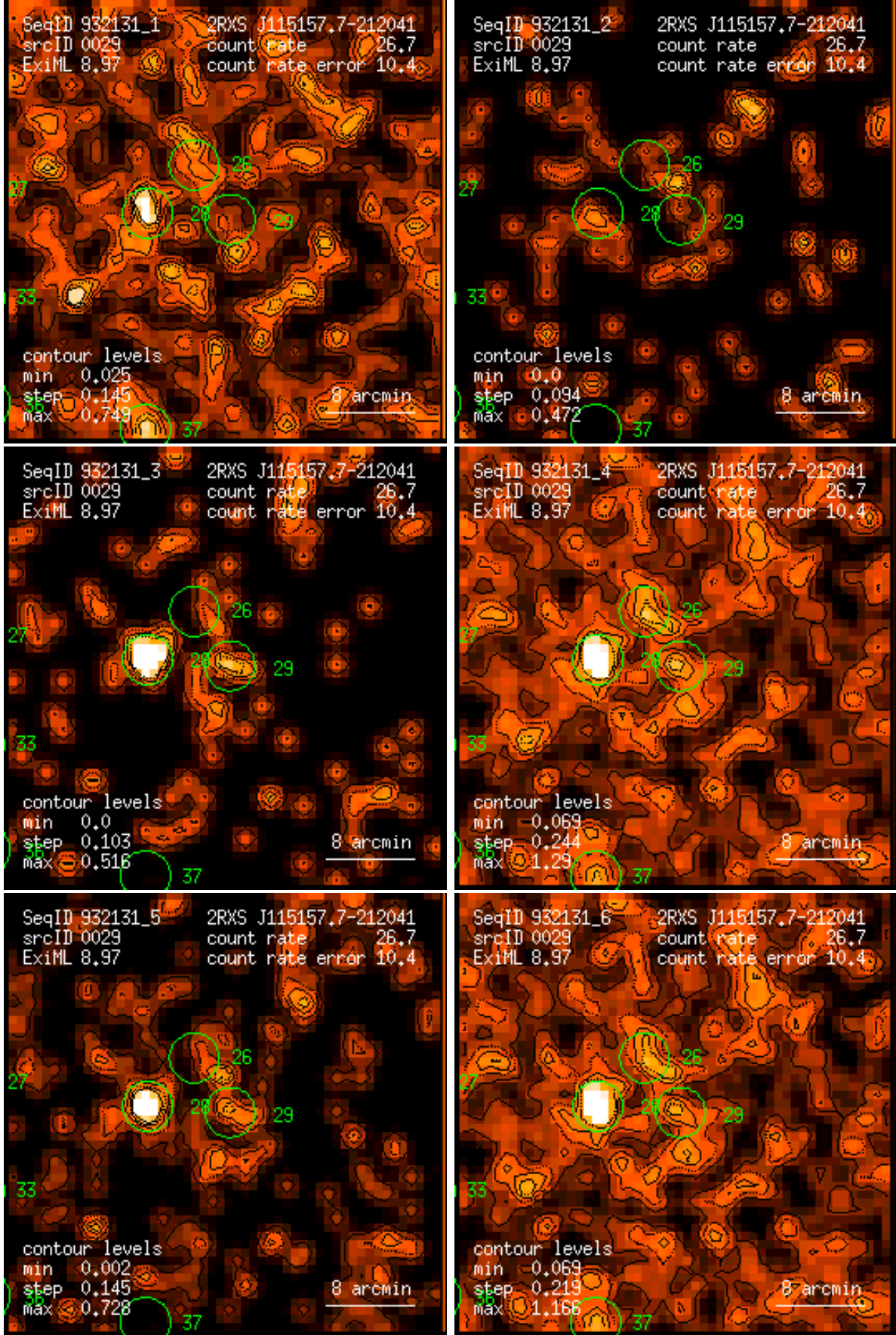
Figure 29: RASS 932131: detection 0029: band rate images, Gaussian filter: (1) PSPC channels 11 – 41, (2) 52 – 90, (3) 91 – 201, (4) 11 – 235, (5) 52 – 201, (6) 11 – 201. Broad band rates in counts/ks. Band rate contour levels in counts/ks/arcmin 2 .
