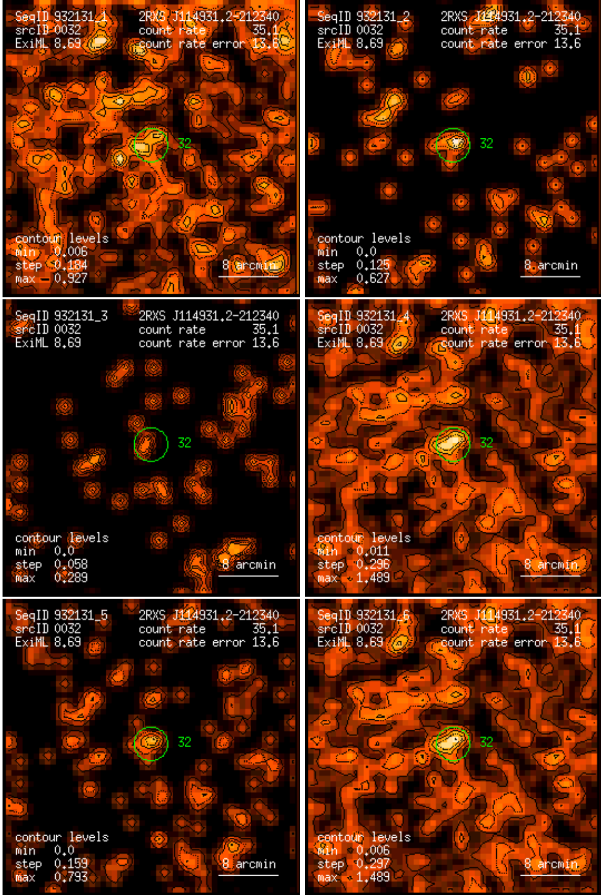
Figure 32: RASS 932131: detection 0032: band rate images, Gaussian filter: (1) PSPC channels 11 – 41, (2) 52 – 90, (3) 91 – 201, (4) 11 – 235, (5) 52 – 201, (6) 11 – 201. Broad band rates in counts/ks. Band rate contour levels in counts/ks/arcmin 2 .
