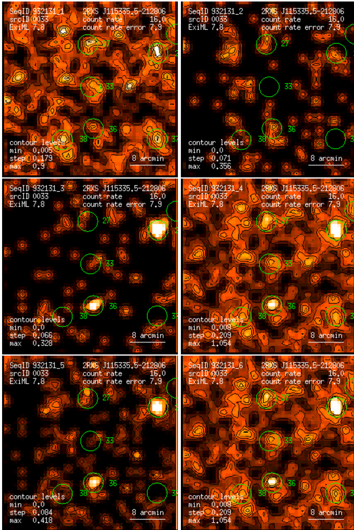
Figure 33: RASS 932131: detection 0033: band rate images, Gaussian filter: (1) PSPC channels 11 – 41, (2) 52 – 90, (3) 91 – 201, (4) 11 – 235, (5) 52 – 201, (6) 11 – 201. Broad band rates in counts/ks. Band rate contour levels in counts/ks/arcmin 2 .
