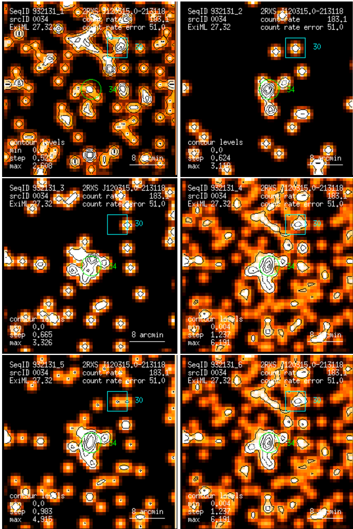
Figure 34: RASS 932131: detection 0034: band rate images, Gaussian filter: (1) PSPC channels 11 – 41, (2) 52 – 90, (3) 91 – 201, (4) 11 – 235, (5) 52 – 201, (6) 11 – 201. Broad band rates in counts/ks. Band rate contour levels in counts/ks/arcmin 2 .
